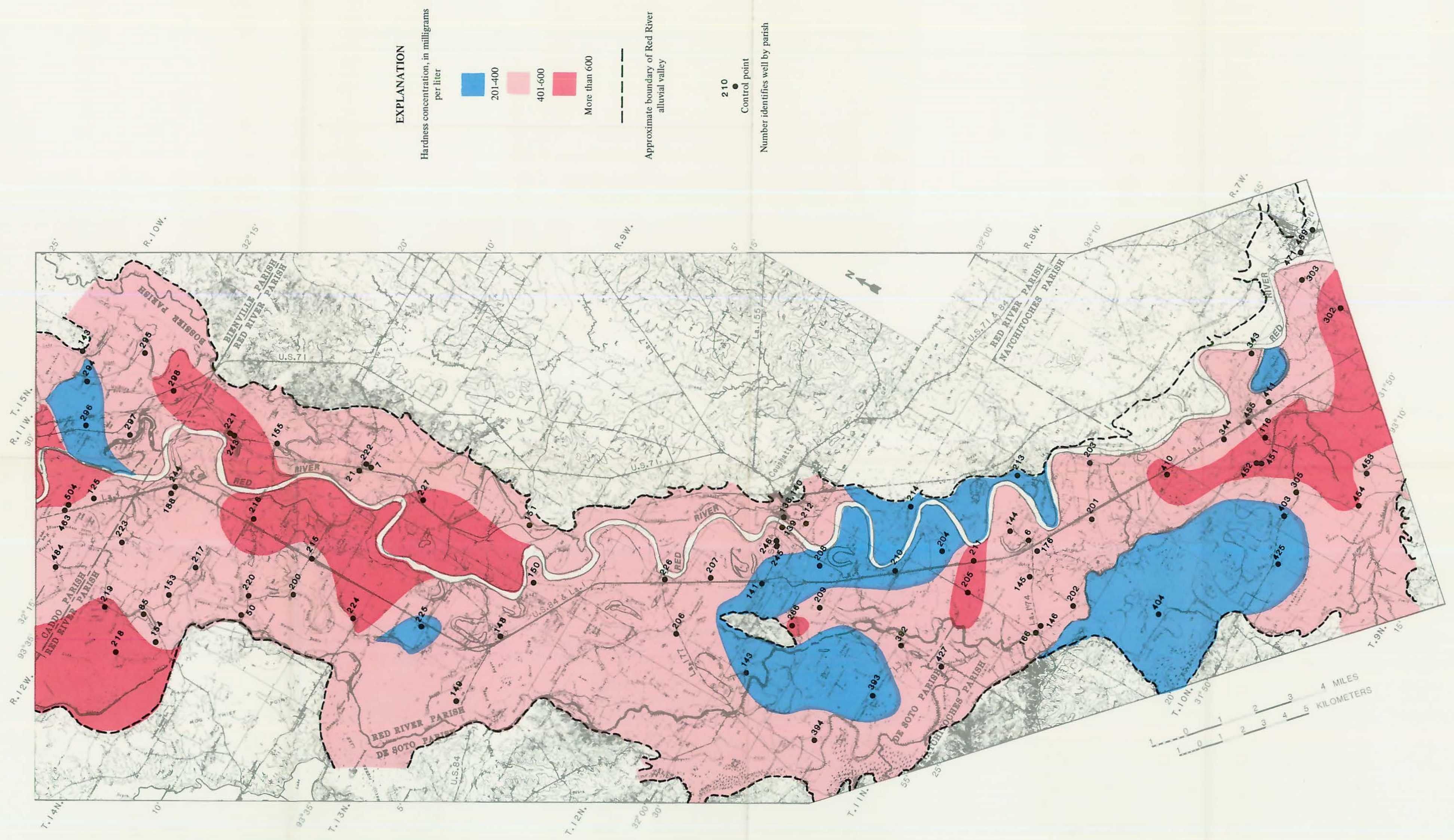
PLATE 3. MAP SHOWING DISTRIBUTION OF HARDNESS IN WATER FROM THE RED RIVER ALLUVIAL AQUIFER, COUSHATTA AREA, LOUISIANA.
