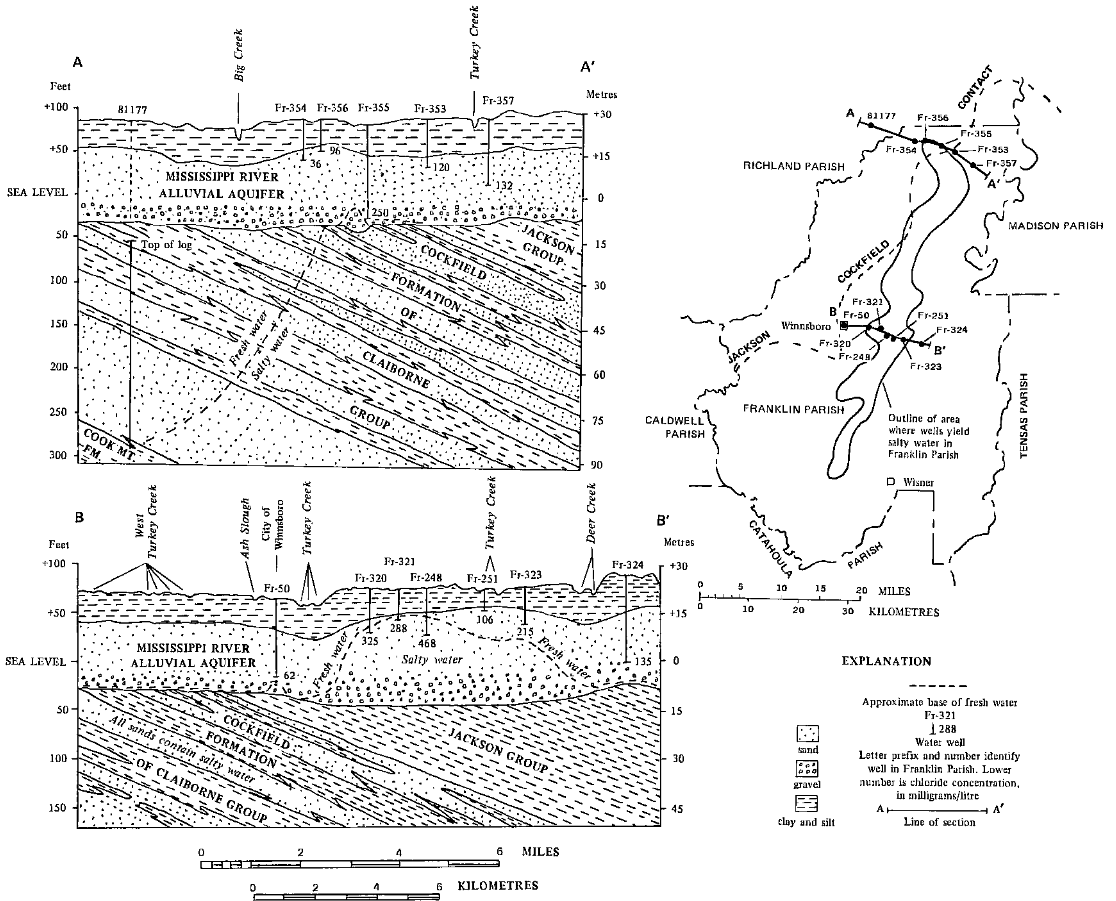
PLATE B. GEOLOGIC SECTIONS SHOWING RELATION BETWEEN FRESH AND SALTY WATER AND MAP SHOWING OUTLINE OF AREA WHERE WELLS YIELD SALTY WATER, FRANKLIN PARISH, LOUISIANA.
