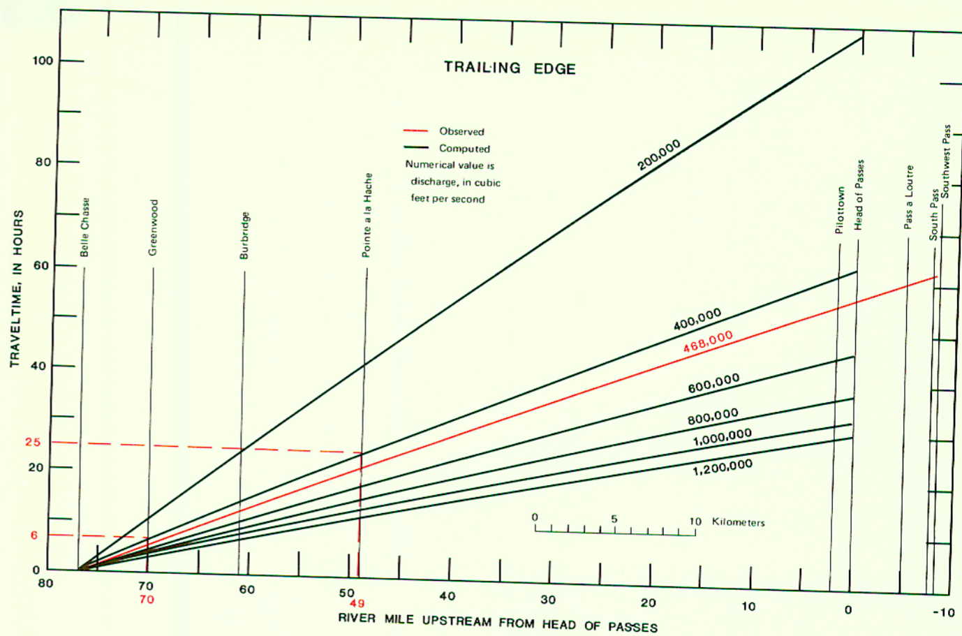
Figure 3.—Curves showing the time of travel of the trailing edge of a tracer cloud at downstream locations along the Mississippi River for different discharge rates.
