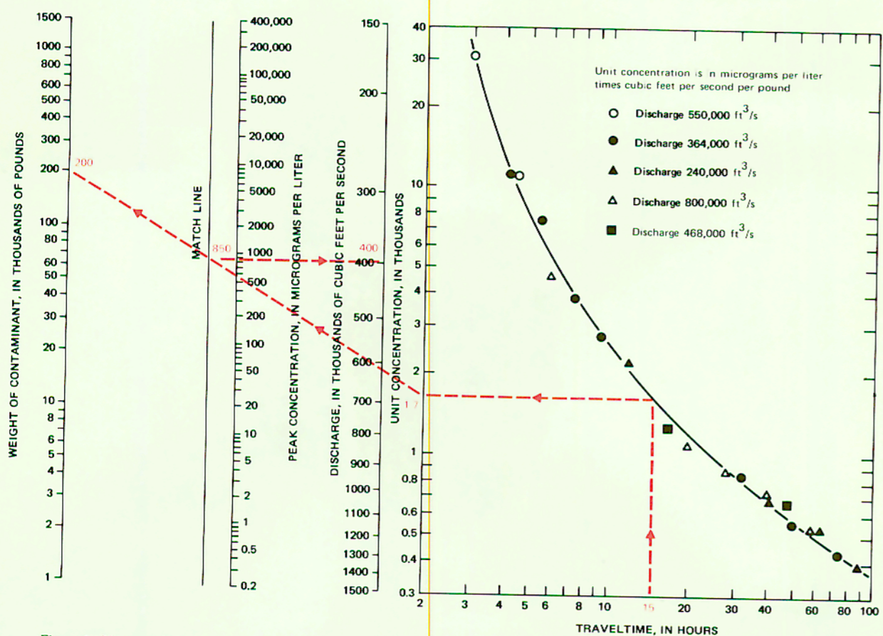
Figure 5.—Nomograph for predicting the peak concentration of a conservative contaminant at downstream sites, by knowing the discharge rate, the elapsed time, and the weight of the contaminant.
