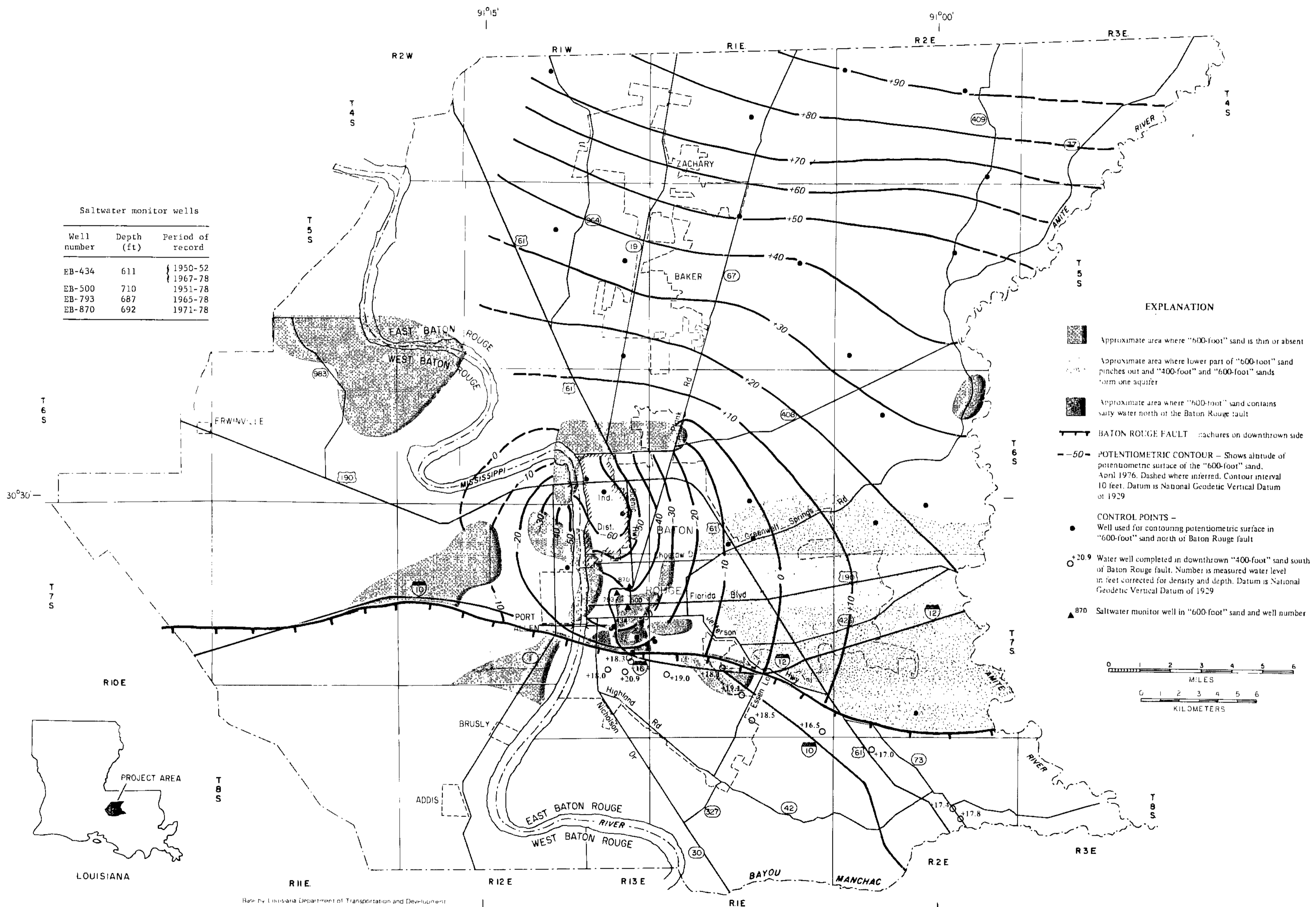
PLATE 3. MAP SHOWING POTENTIOMETRIC SURFACE OF THE "600-FOOT" SAND, APRIL 1976, BATON ROUGE AREA, LOUISIANA.
