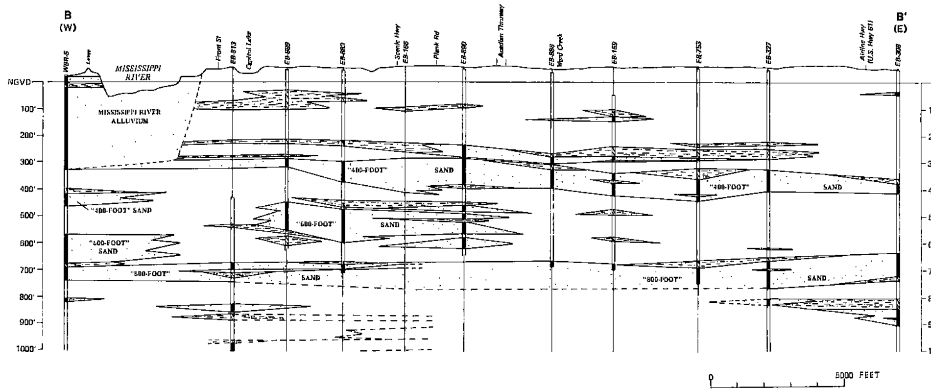
B. East-west section across the southern end of the industrial district.
