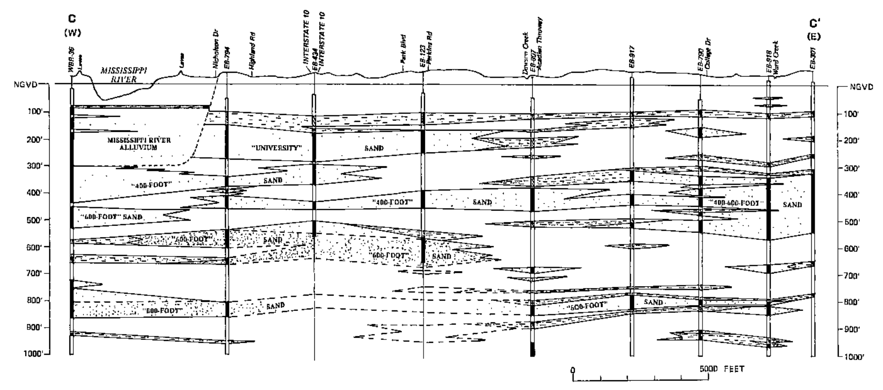
C. East-west section along the north side of the Baton Rouge fault.
