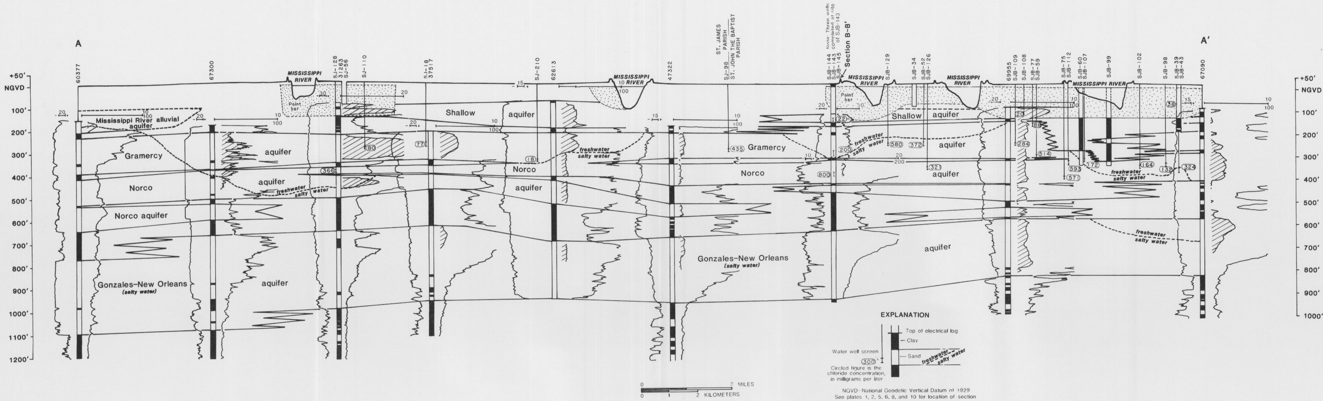
PLATE 3. GEOHYDROLOGIC SECTION A-A', GRAMERCY AREA, LOUISIANA.
