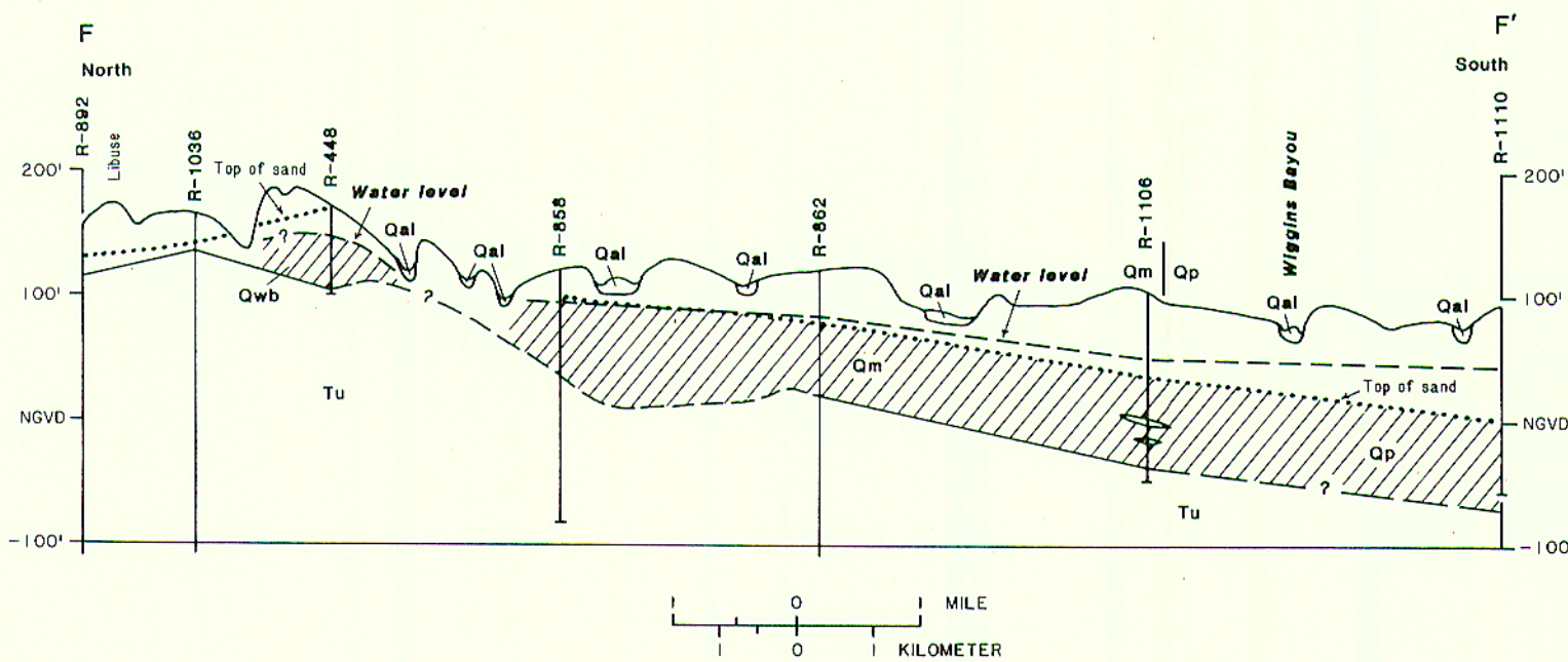
B. North-south geohydrologic section.
