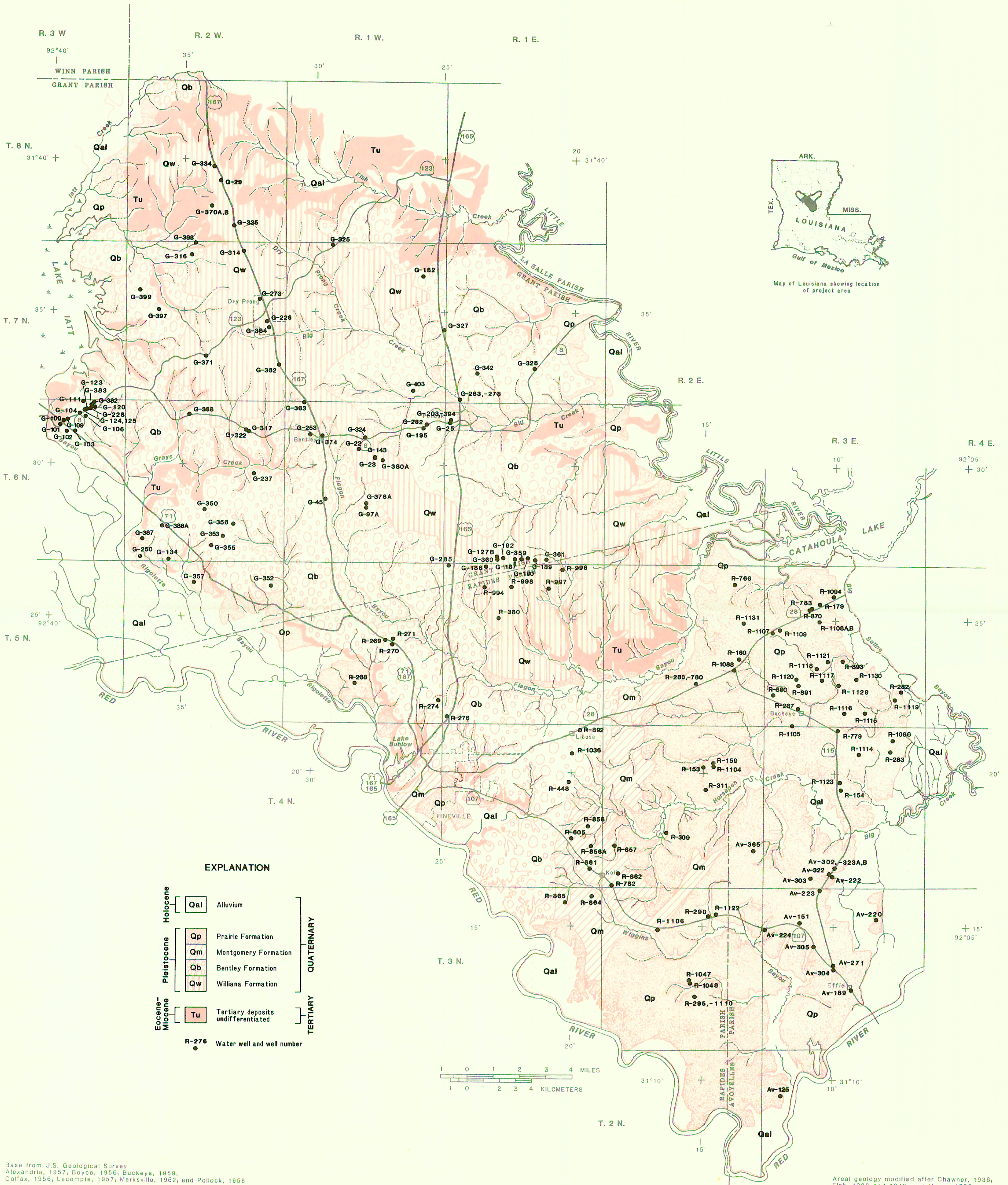
PLATE 2C. MAP SHOWING LOCATION OF SELECTED WELLS AND AREAL GEOLOGY OF THE CENTRAL PART OF THE PROJECT AREA, CENTRAL LOUISIANA.
