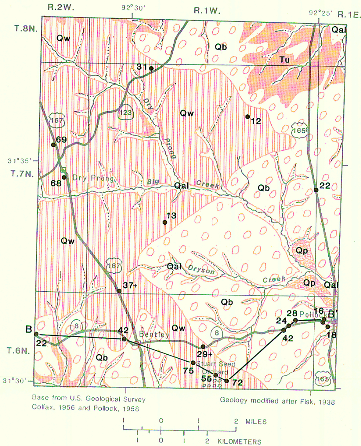
A. Surface geology and saturated-sand thickness.
