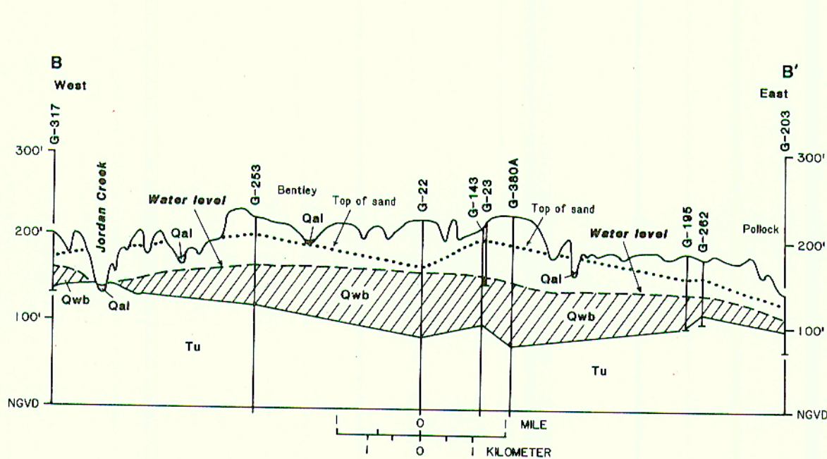
B. West-east geohydrologic section.
