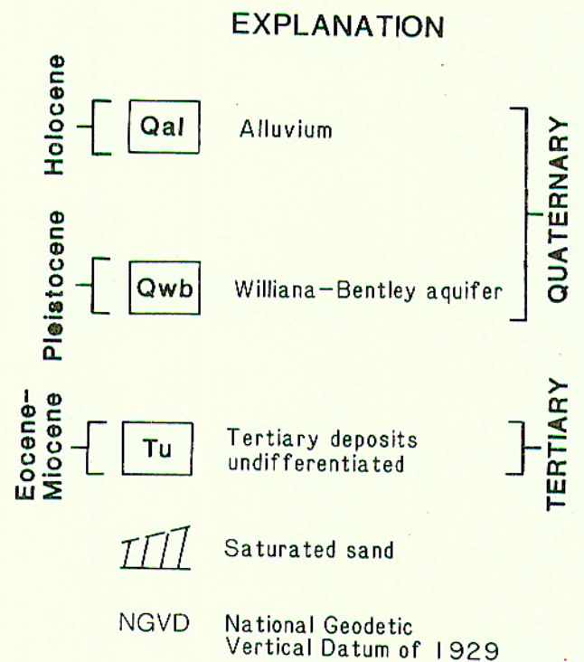
PLATE 7. MAP AND SECTION SHOWING GEOLOGY AND SATURATED-SAND THICKNESS, BENTLEY-DRY PRONG-POLLOCK AREA, GRANT PARISH, LOUISIANA.
