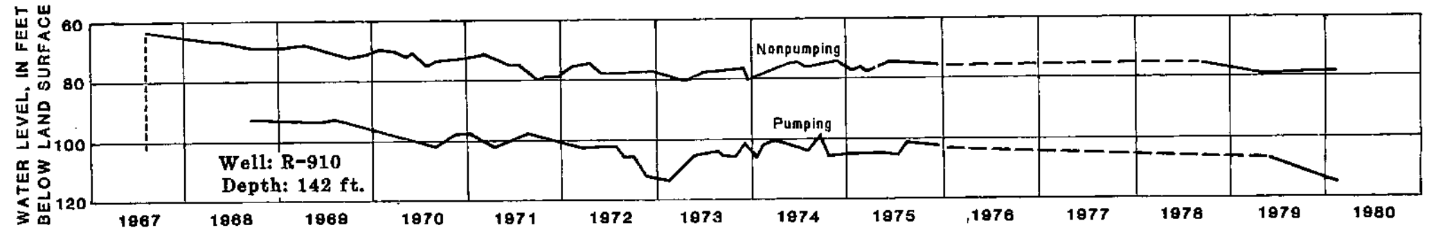
C. Terrace deposits
