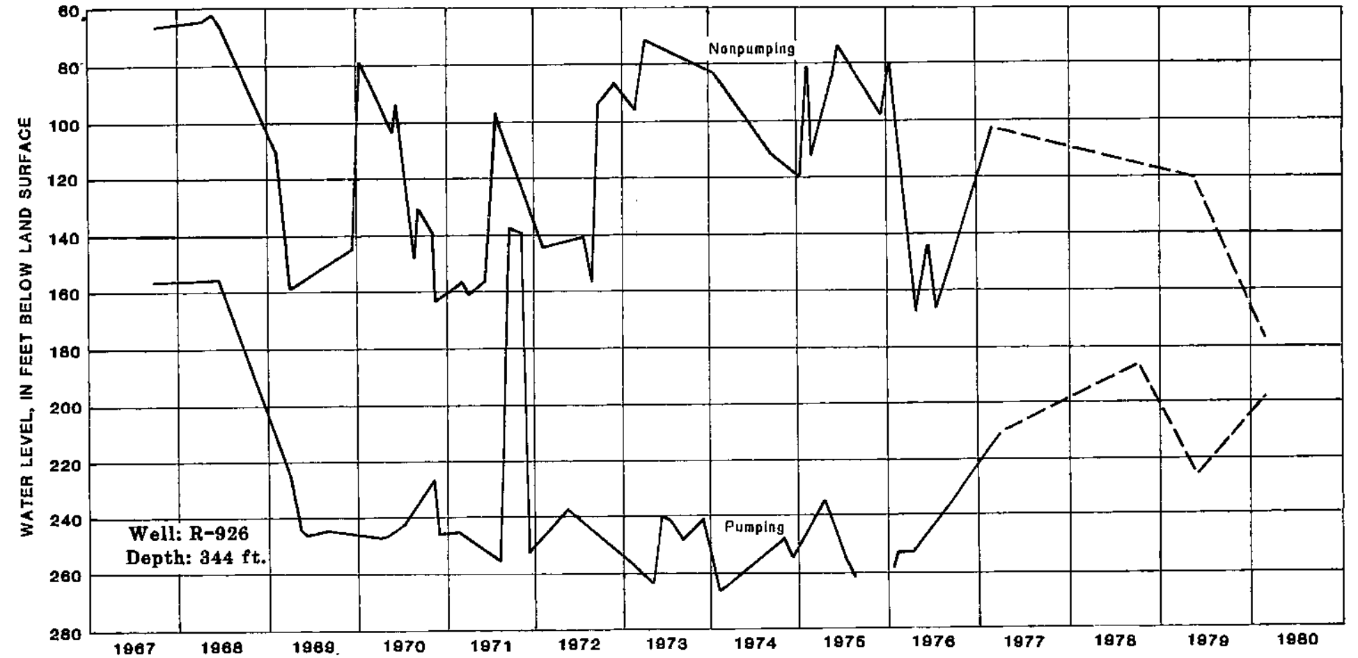
D. Blounts Creek Member of Fleming Formation
