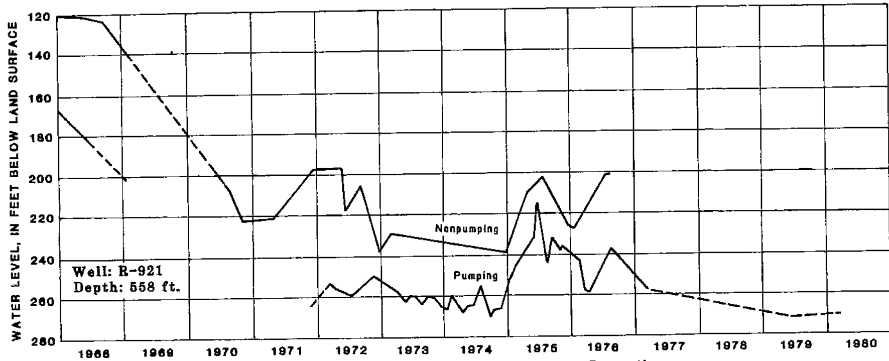
B. Williamson Creek Member of Fleming Formation
