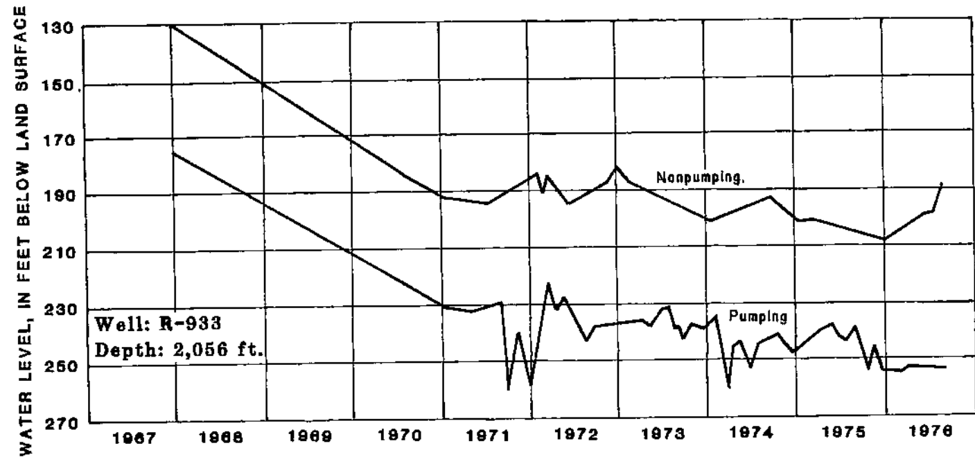
A. Carnahan Bayou Member of Fleming Formation
