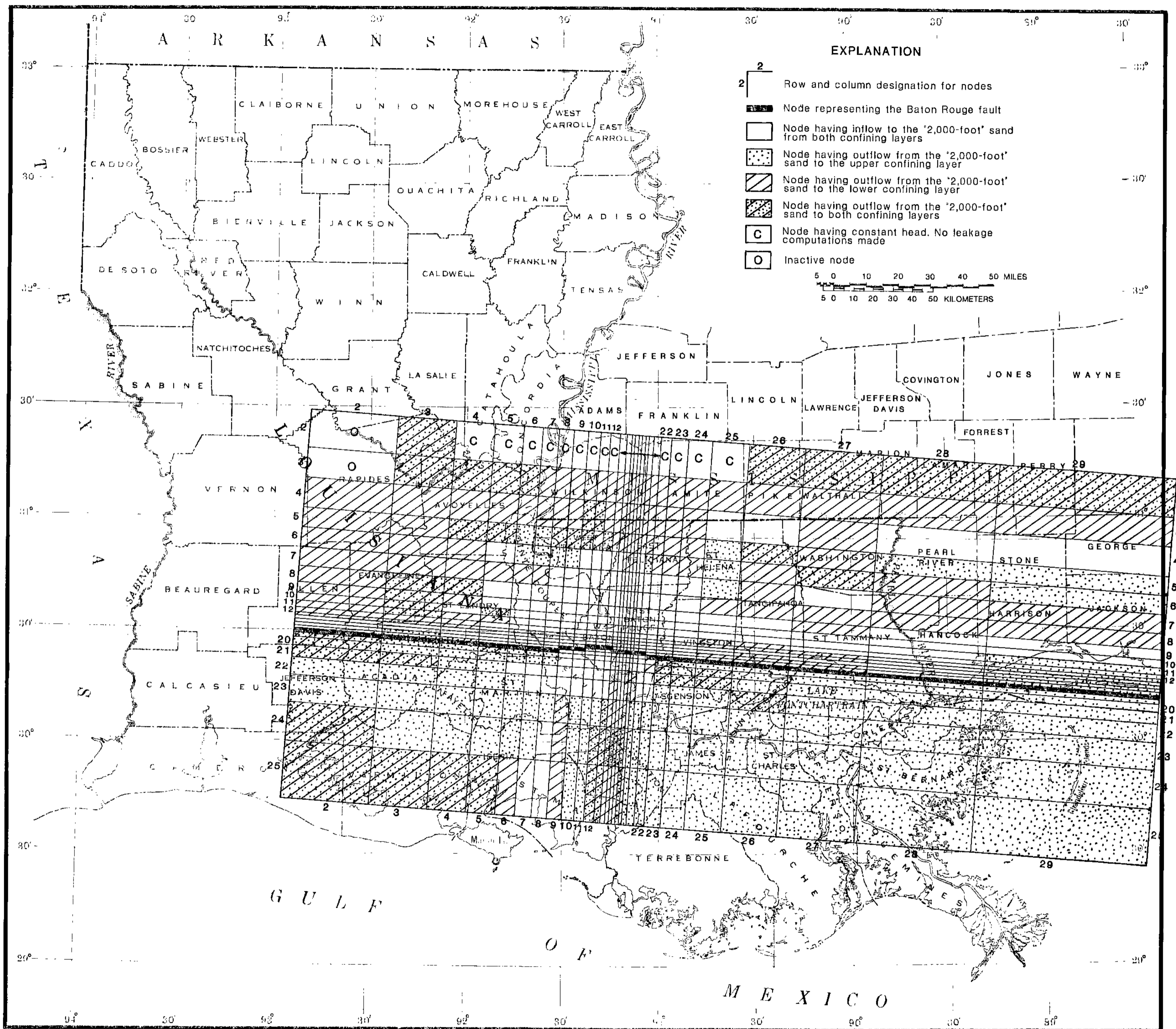
PLATE 4. MAP SHOWING AREAS OF INFLOW TO AND OUTFLOW FROM THE '2,000-FOOT' SAND AND CONFINING LAYERS COMPUTED BY THE DETAILED THREE-DIMENSIONAL MODEL, SOUTHEASTERN LOUISIANA AND SOUTHWESTERN MISSISSIPPI.
