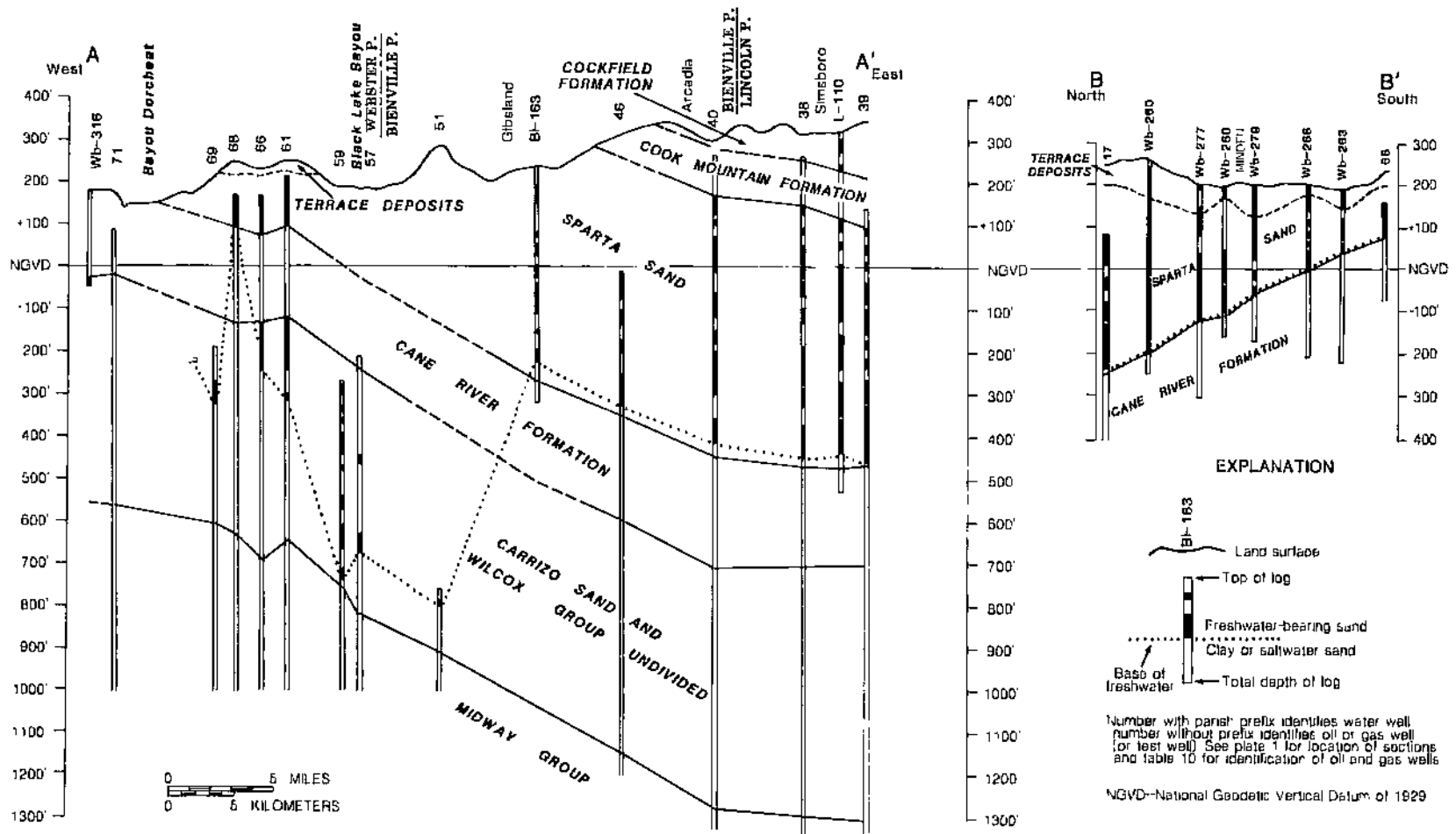
PLATE 3. GEOLOGIC SECTIONS OF THE ARCADIA-MINDEN AREA, LOUISIANA.
