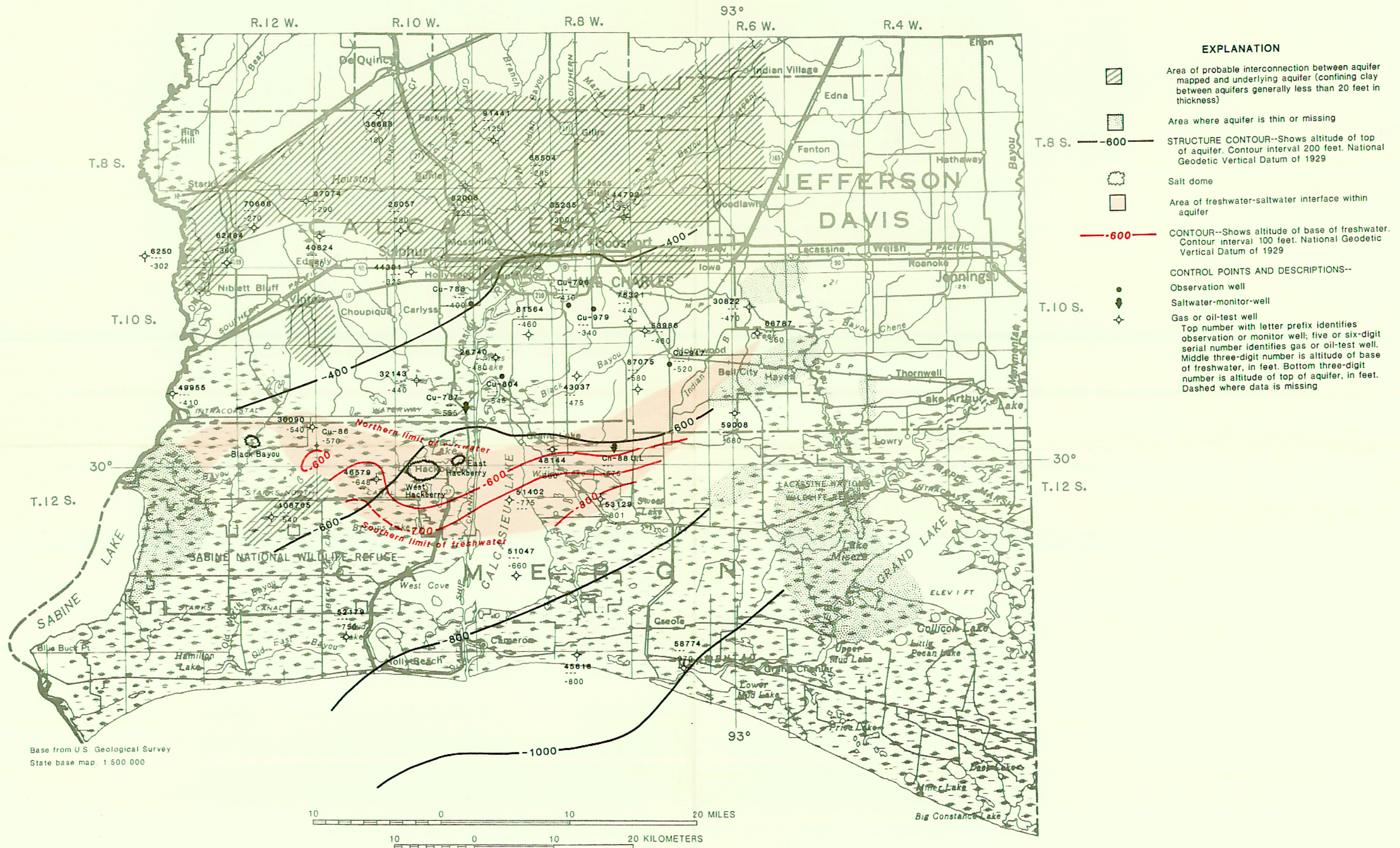
PLATE 4. ALTITUDE OF THE BASE OF FRESHWATER AND STRUCTURE CONTOURS ON THE TOP OF THE '500-FOOT' SAND OF THE CHICOT AQUIFER SYSTEM IN SOUTHWESTERN LOUISIANA.
