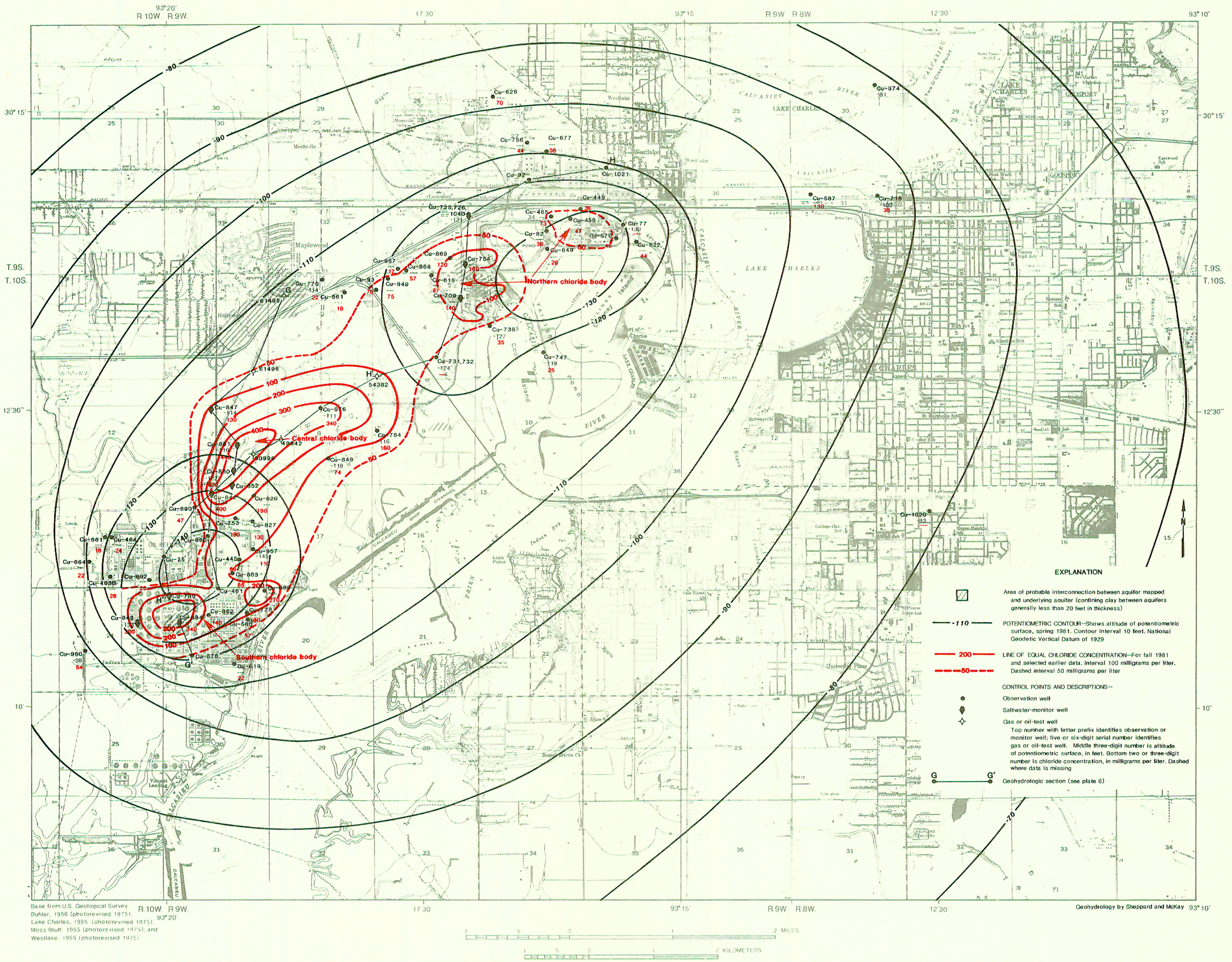
PLATE 5. CONCENTRATION OF HIGH-CHLORIDE WATER IN (FALL 1981) AND POTENTIOMETRIC SURFACE OF THE "500-FOOT" SAND IN (SPRING 1981) OF THE CHICOT AQUIFER SYSTEM IN THE LAKE CHARLES INDUSTRIAL AREA.
