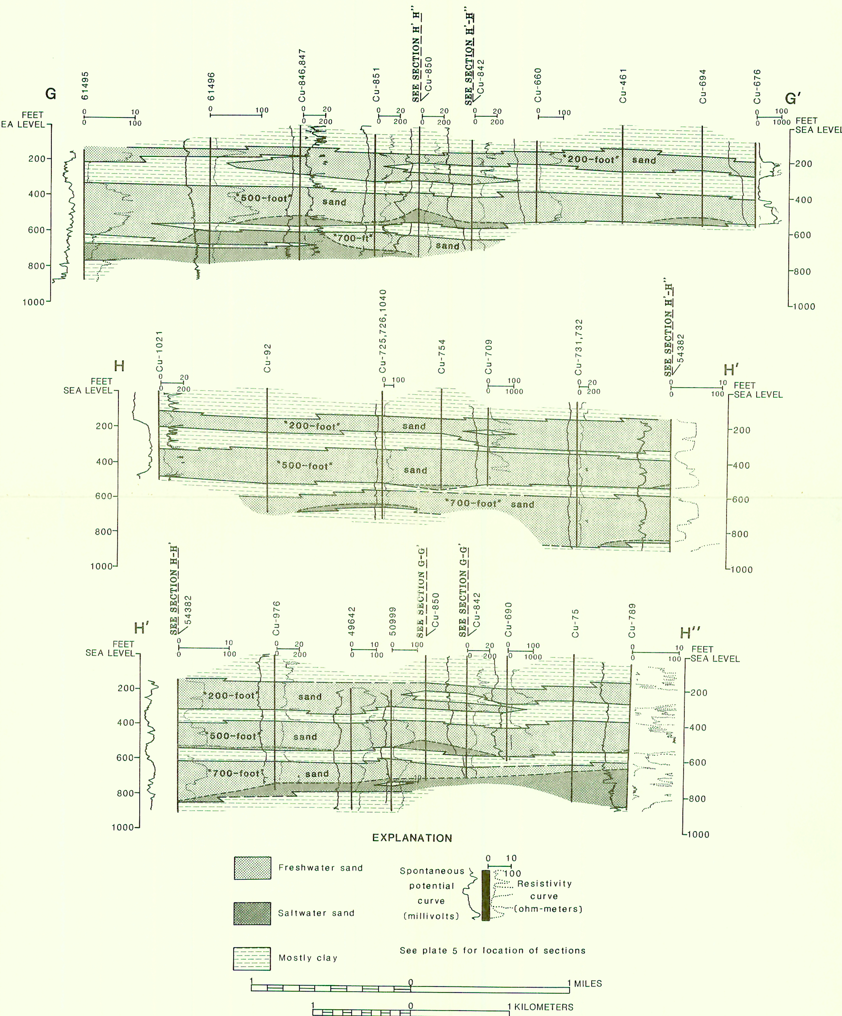
PLATE 6. GEOHYDROLOGIC SECTIONS THROUGH THE CHICOT AQUIFER SYSTEM IN THE LAKE CHARLES INDUSTRIAL AREA, LOUISIANA.
