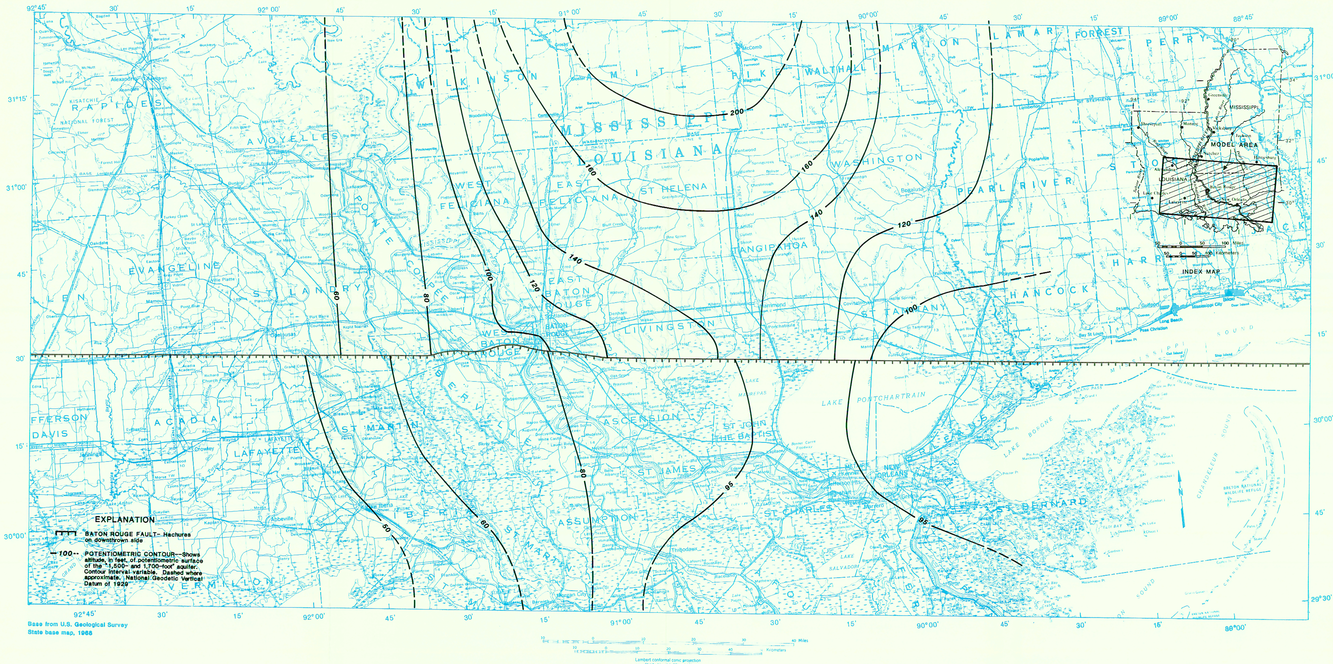
PLATE 10. COMPUTED STEADY-STATE POTENTIOMETRIC SURFACE OF THE "1,500- AND 1,700-FOOT" AQUIFER (PRE-1920), SOUTHEASTERN LOUISIANA AND SOUTHWESTERN MISSISSIPPI.
