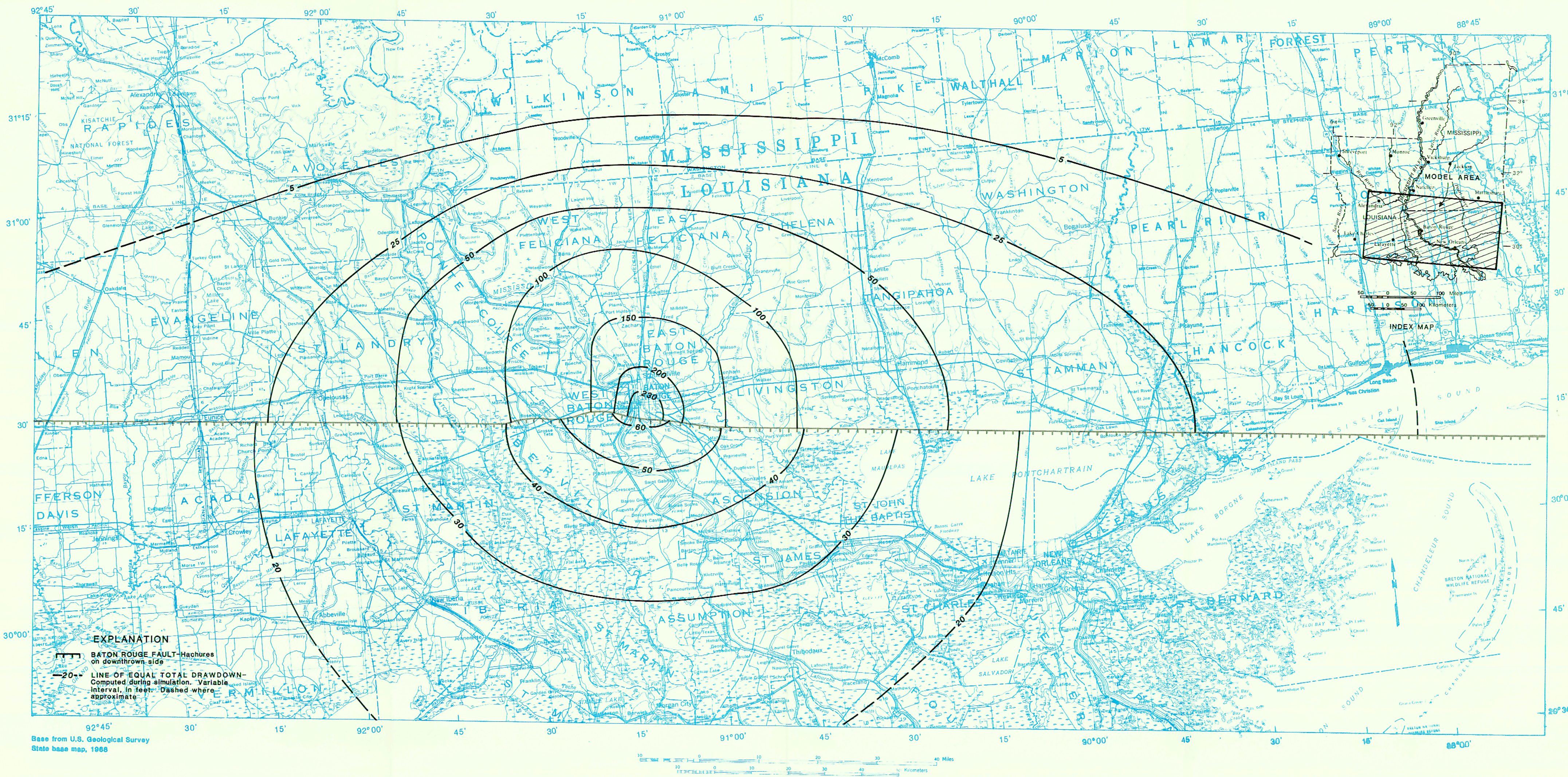
PLATE 6. COMPUTED TOTAL DRAWDOWN FOR A 5-PERCENT INCREASE IN PUMPING FROM THE "1,500- and 1,700-FOOT" AQUIFER FOR EACH OF SIX 5-YEAR PERIODS (TOTAL PERIOD 1920-2009), SOUTHEASTERN LOUISIANA AND SOUTHWESTERN MISSISSIPPI.
