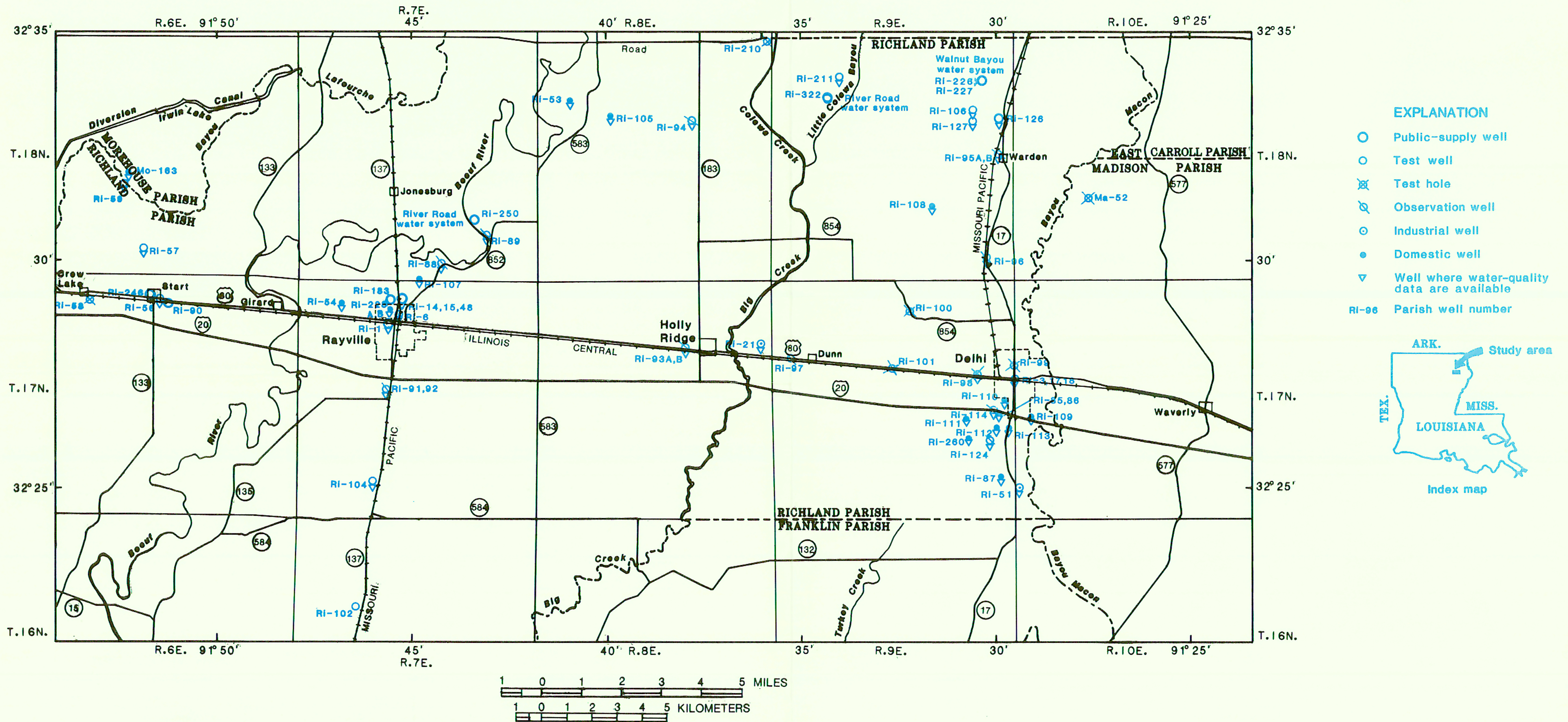
PLATE 1. LOCATION OF SELECTED WELLS AND TEST HOLES IN THE RAYVILLE-DELHI AREA, NORTHEASTERN LOUISIANA.
