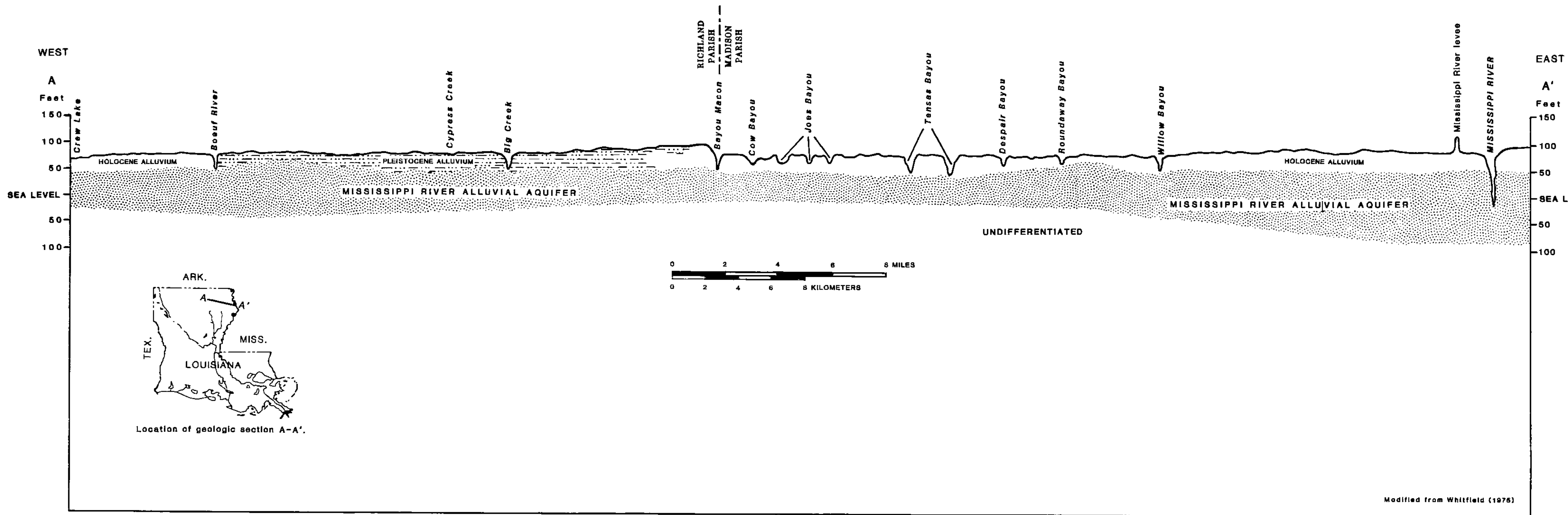
GEOLOGIC SECTION ACROSS THE MISSISSIPPI RIVER ALLUVIAL VALLEY BETWEEN CREW LAKE, LOUISIANA AND THE MISSISSIPPI RIVER.
