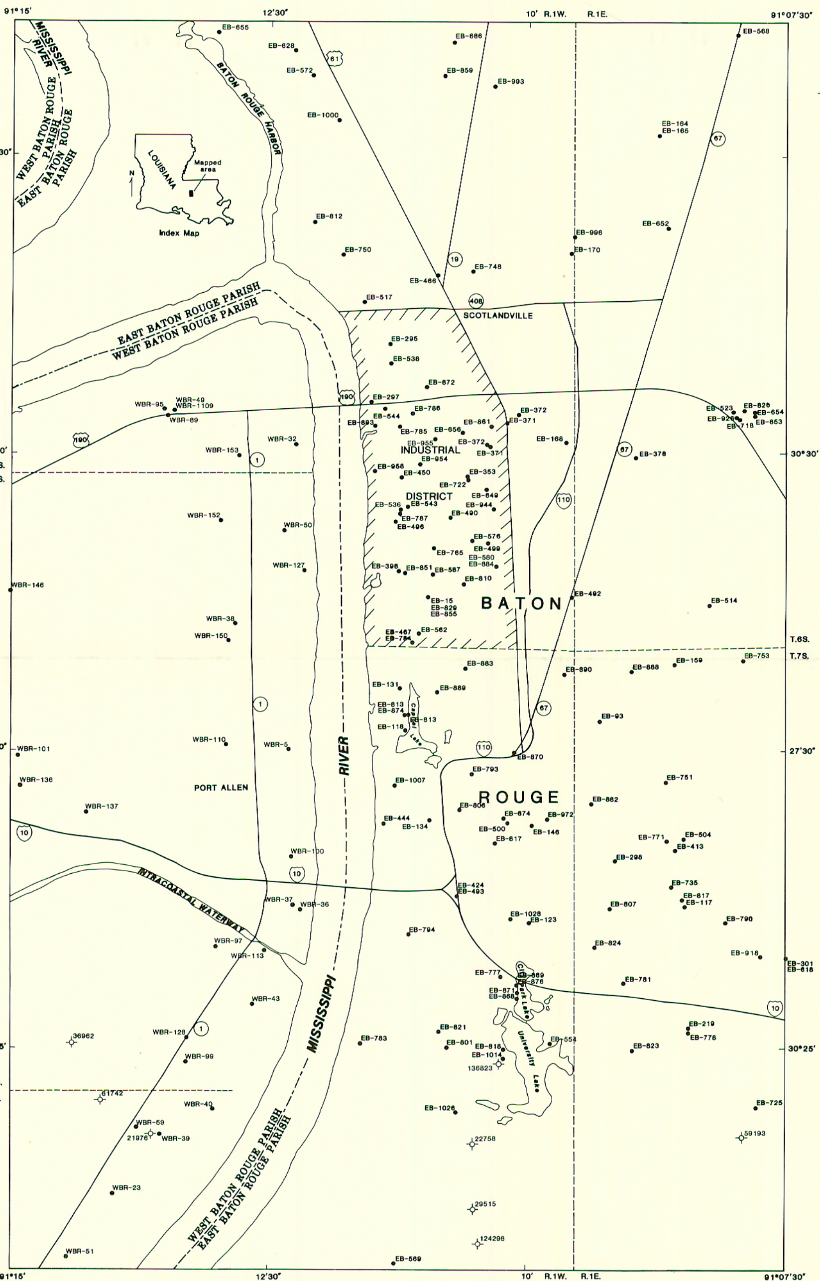
PLATE 1. LOCATION OF SITES WITH WELL LOGS IN THE BATON ROUGE INDUSTRIAL DISTRICT AND THE SURROUNDING AREA, LOUISIANA.
