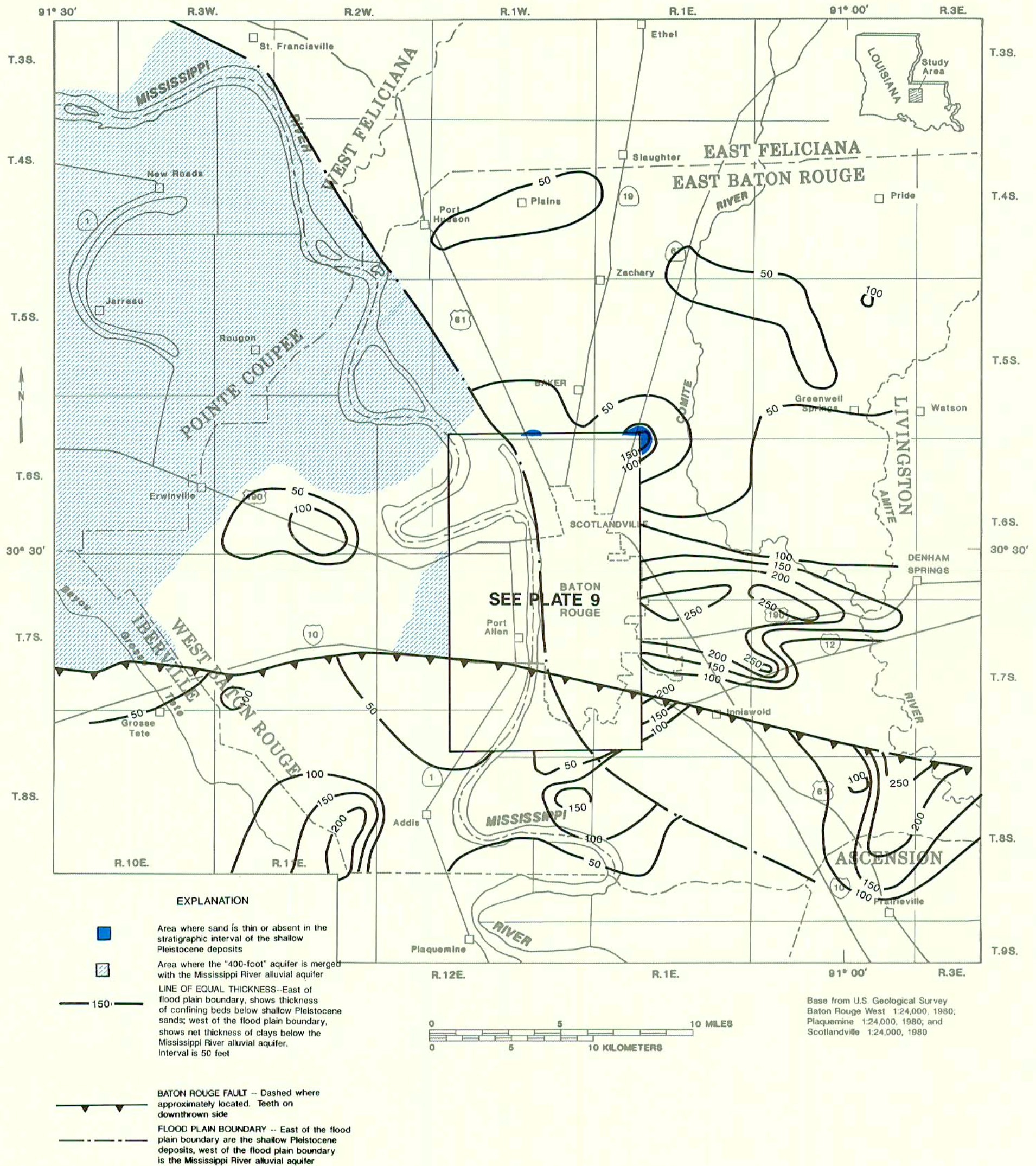
PLATE 10. CONFINING BED THICKNESS BELOW SHALLOW PLEISTOCENE DEPOSITS AND THE MISSISSIPPI RIVER ALLUVIAL AQUIFER IN EAST BATON ROUGE PARISH AND THE SURROUNDING PARISHES, LOUISIANA.
