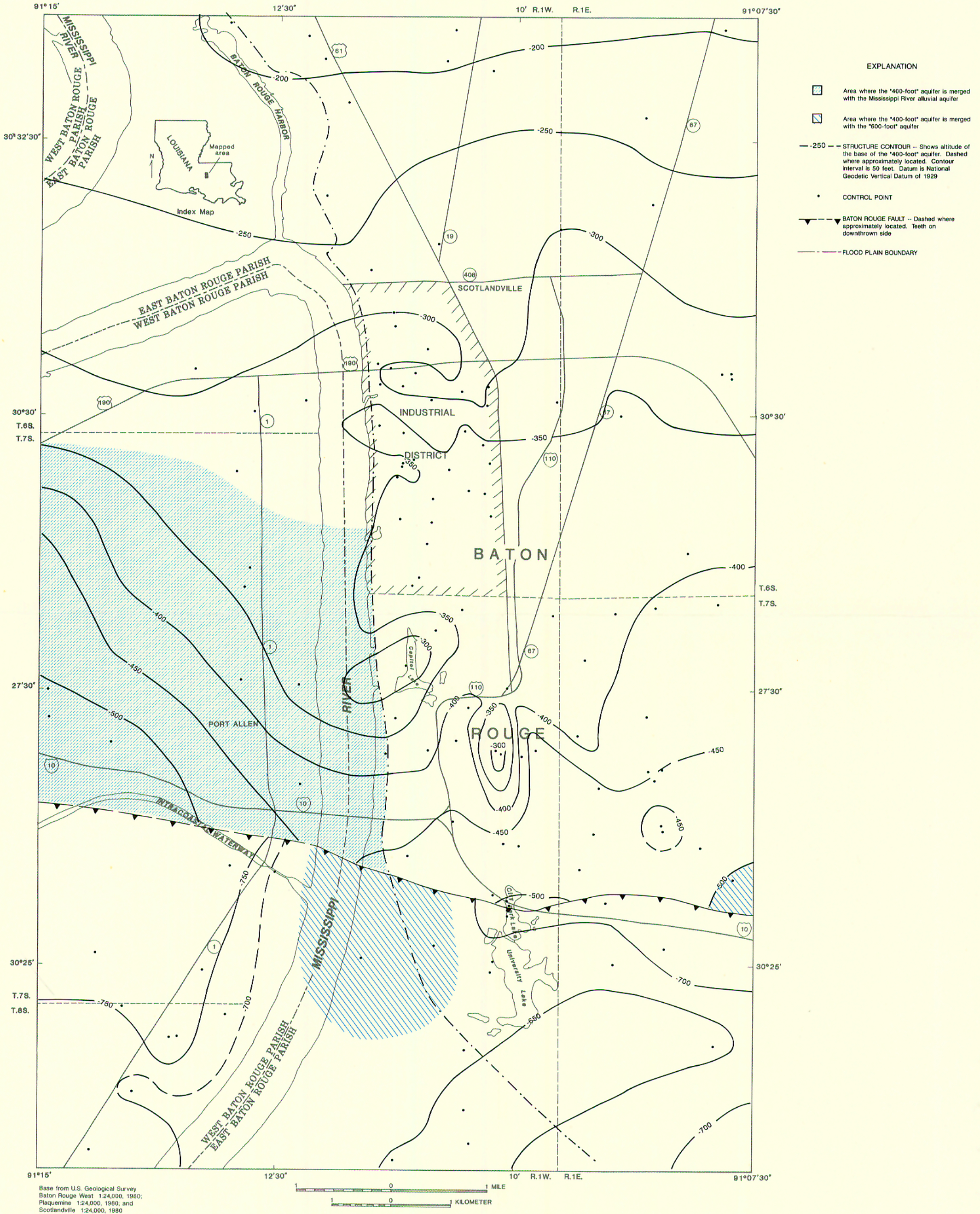
PLATE 11. ALTITUDE OF THE BASE OF THE "400-FOOT" AQUIFER IN THE BATON ROUGE INDUSTRIAL DISTRICT AND THE SURROUNDING AREA, LOUISIANA.
