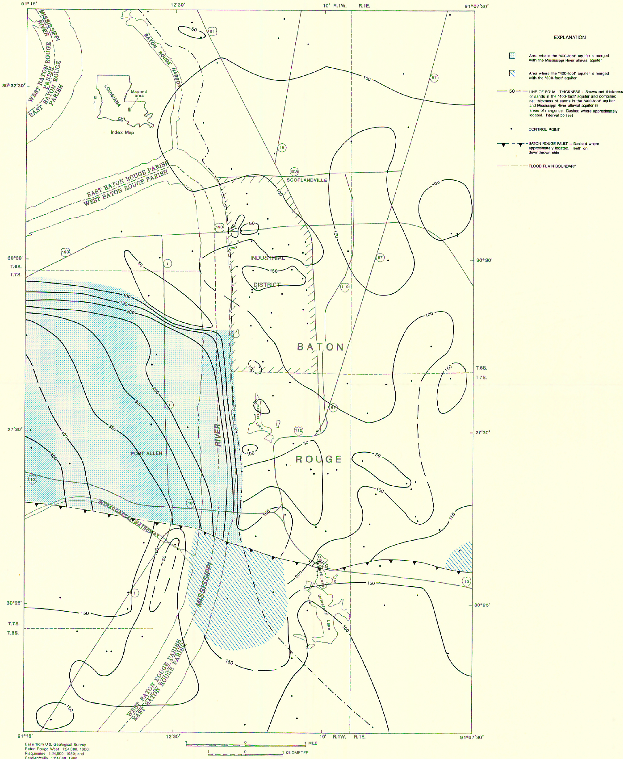
PLATE 13. NET SAND THICKNESS OF THE "400-FOOT" AQUIFER IN THE BATON ROUGE INDUSTRIAL DISTRICT AND THE SURROUNDING AREA, LOUISIANA.
