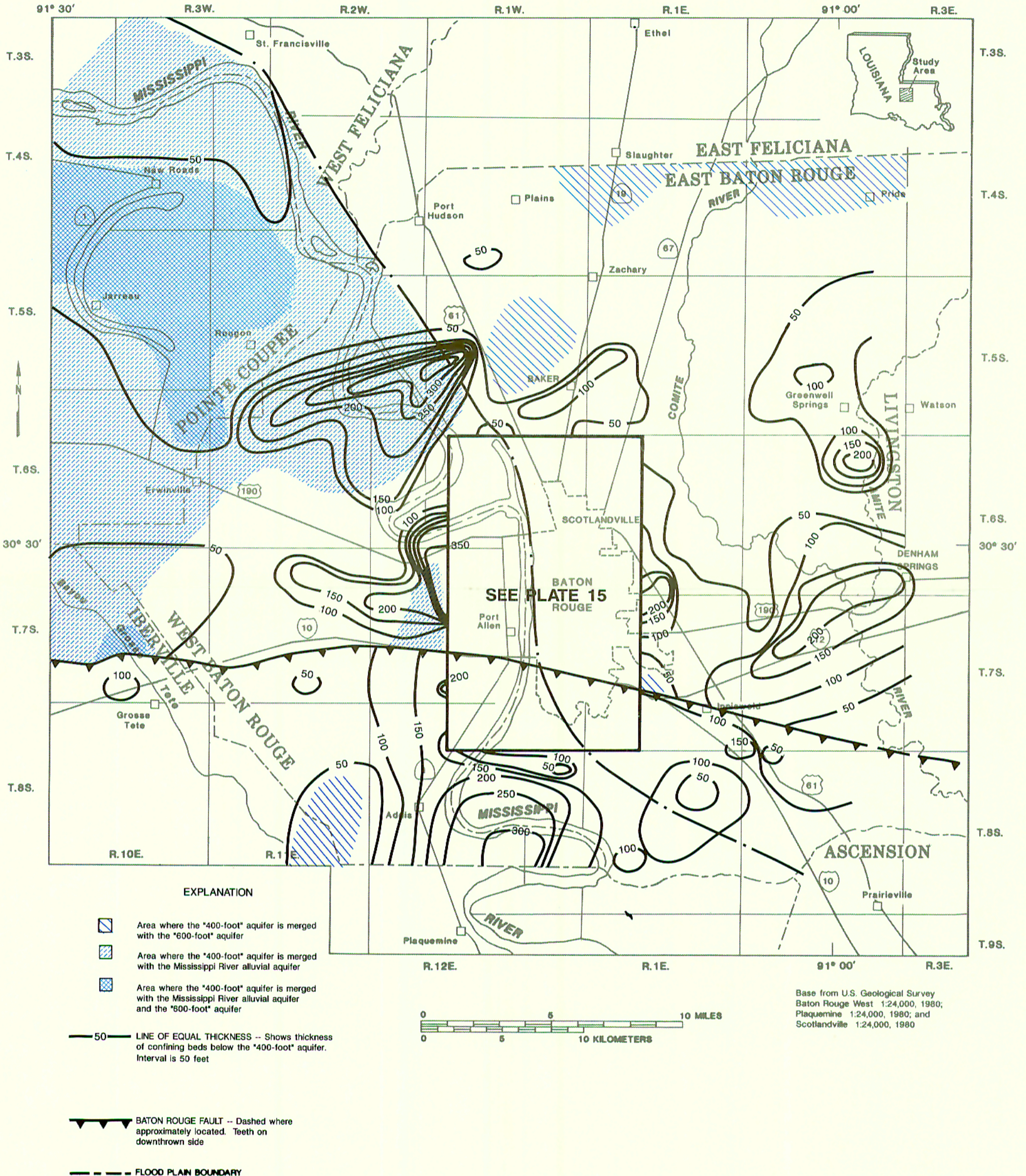
PLATE 16. CONFINING BED THICKNESS BELOW THE "400-FOOT" AQUIFER IN EAST BATON ROUGE PARISH AND SURROUNDING PARISHES, LOUISIANA.
