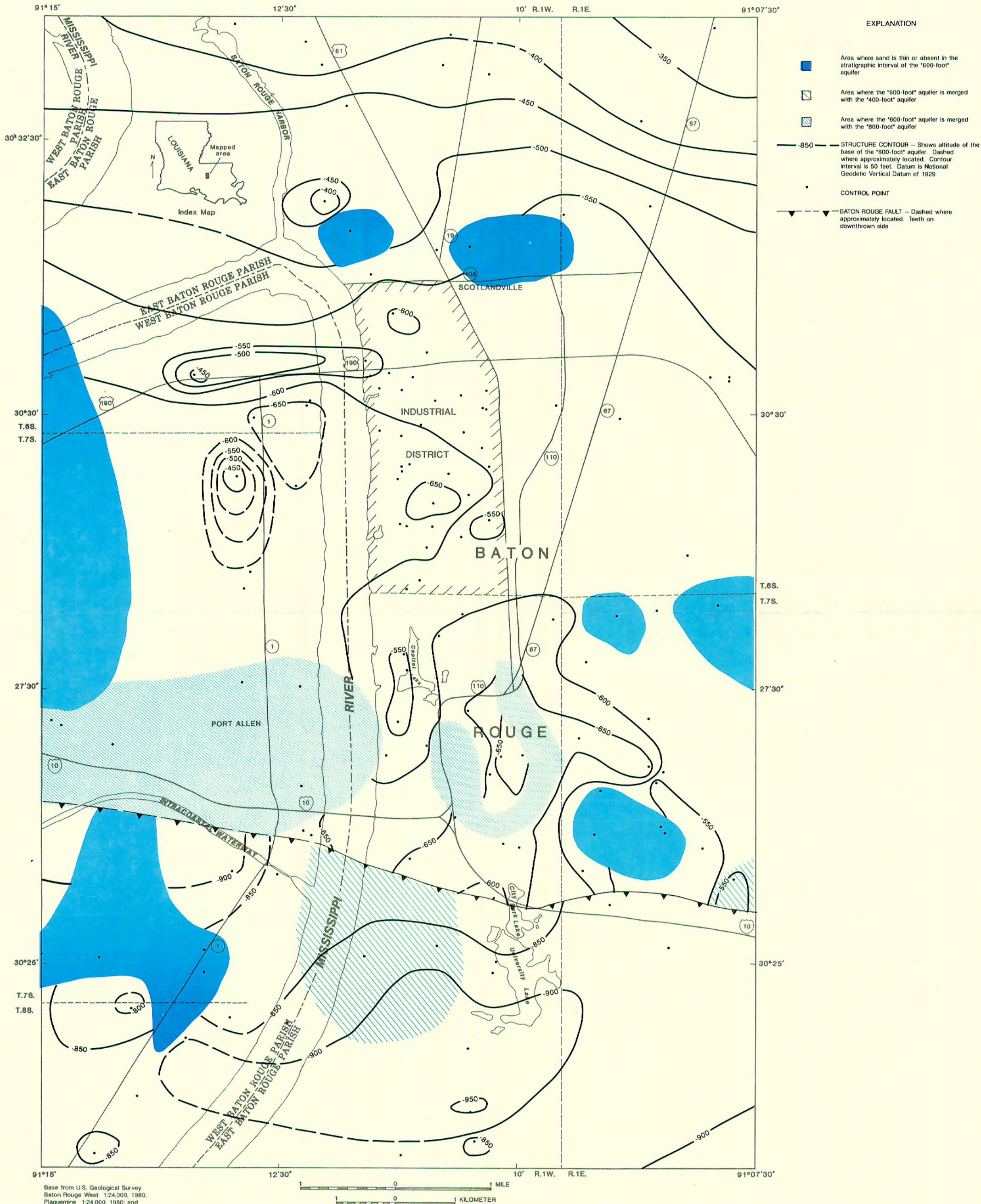
PLATE 17. ALTITUDE OF THE BASE OF THE "600-FOOT" AQUIFER IN THE BATON ROUGE INDUSTRIAL DISTRICT AND THE SURROUNDING AREA, LOUISIANA.
