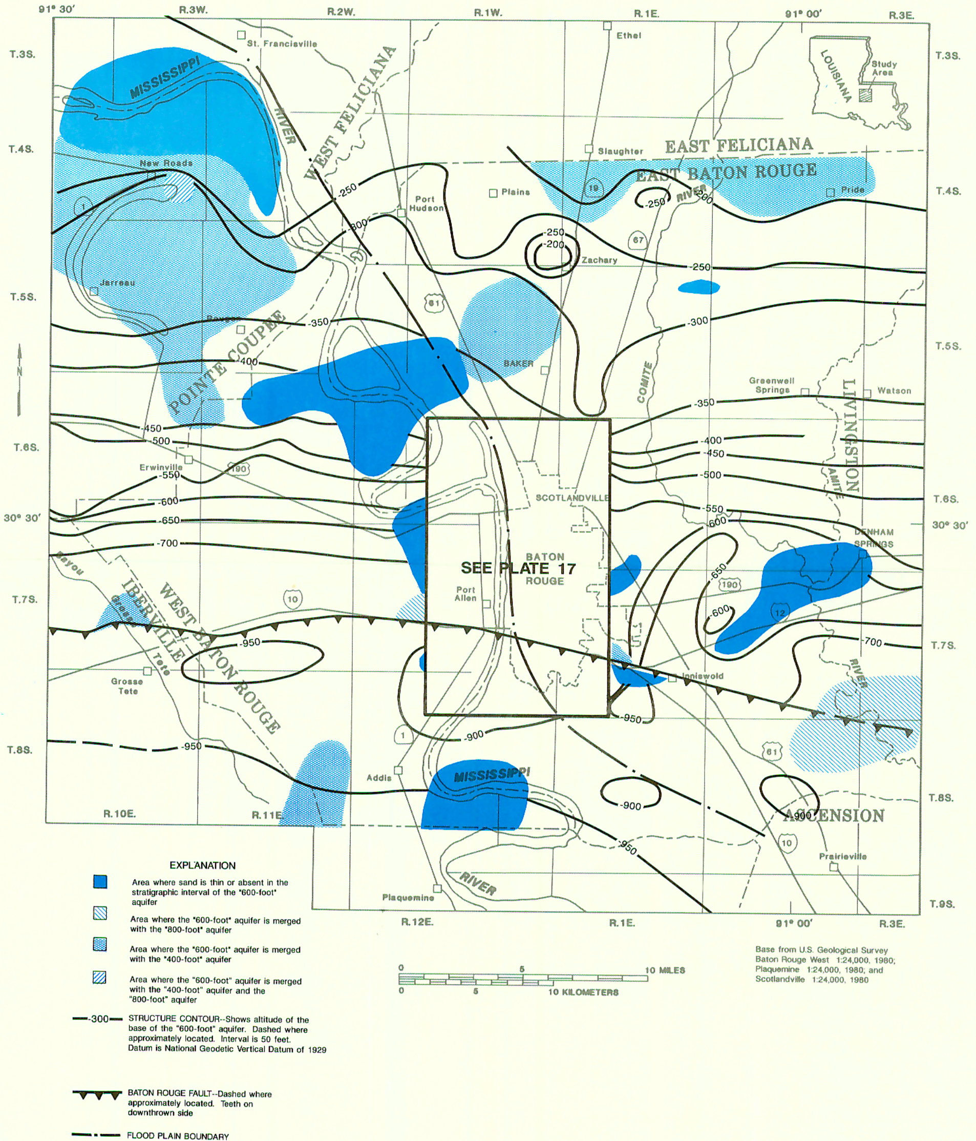
PLATE 18. ALTITUDE OF THE BASE OF THE "600-FOOT" AQUIFER IN EAST BATON ROUGE PARISH AND SURROUNDING PARISHES, LOUISIANA.
