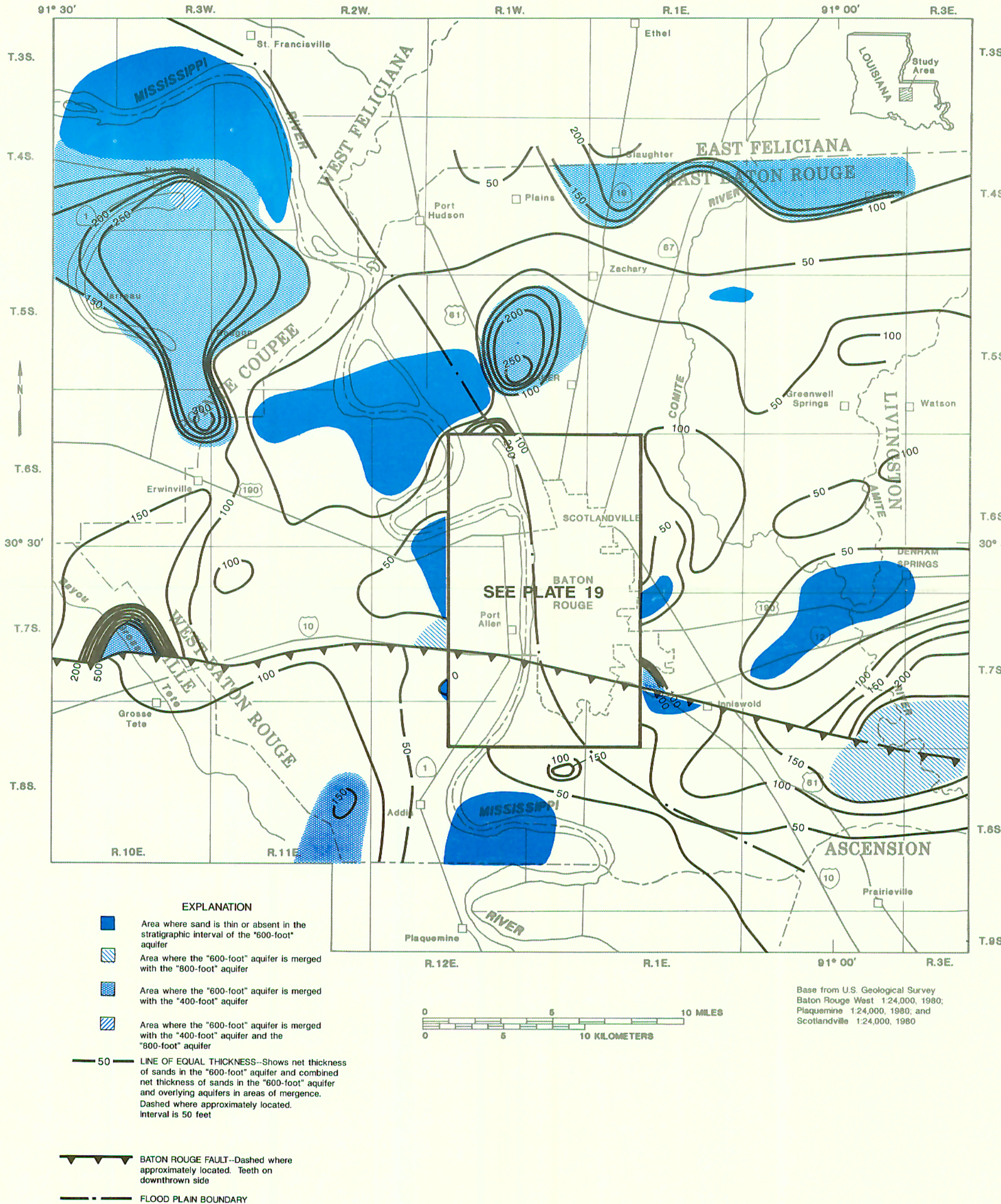
PLATE 20. NET SAND THICKNESS OF THE "600-FOOT" AQUIFER IN EAST BATON ROUGE PARISH AND SURROUNDING PARISHES, LOUISIANA.
