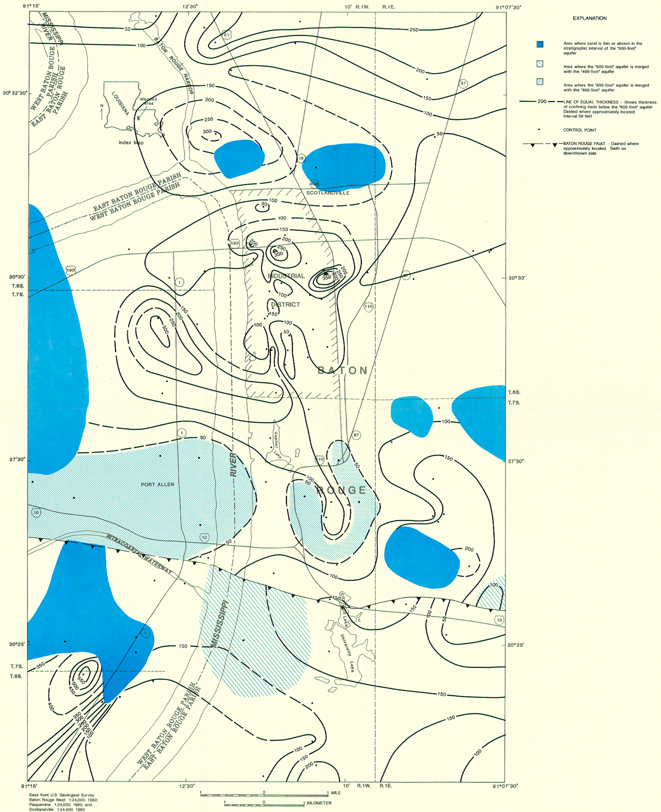
PLATE 21. CONFINING BED THICKNESS BELOW THE "600-FOOT" AQUIFER IN THE BATON ROUGE INDUSTRIAL DISTRICT AND THE SURROUNDING AREA, LOUISIANA.
