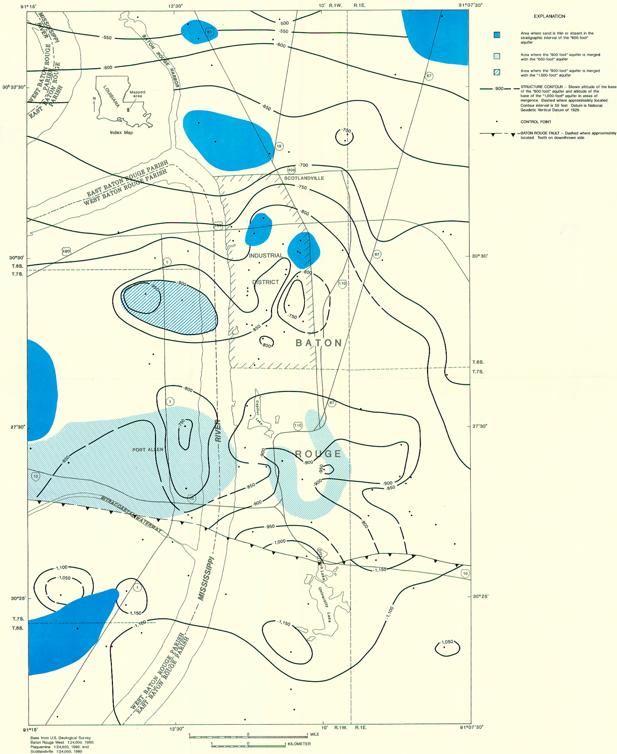
PLATE 23. ALTITUDE OF THE BASE OF THE "800-FOOT" AQUIFER IN THE BATON ROUGE INDUSTRIAL DISTRICT AND THE SURROUNDING AREA, LOUISIANA.
