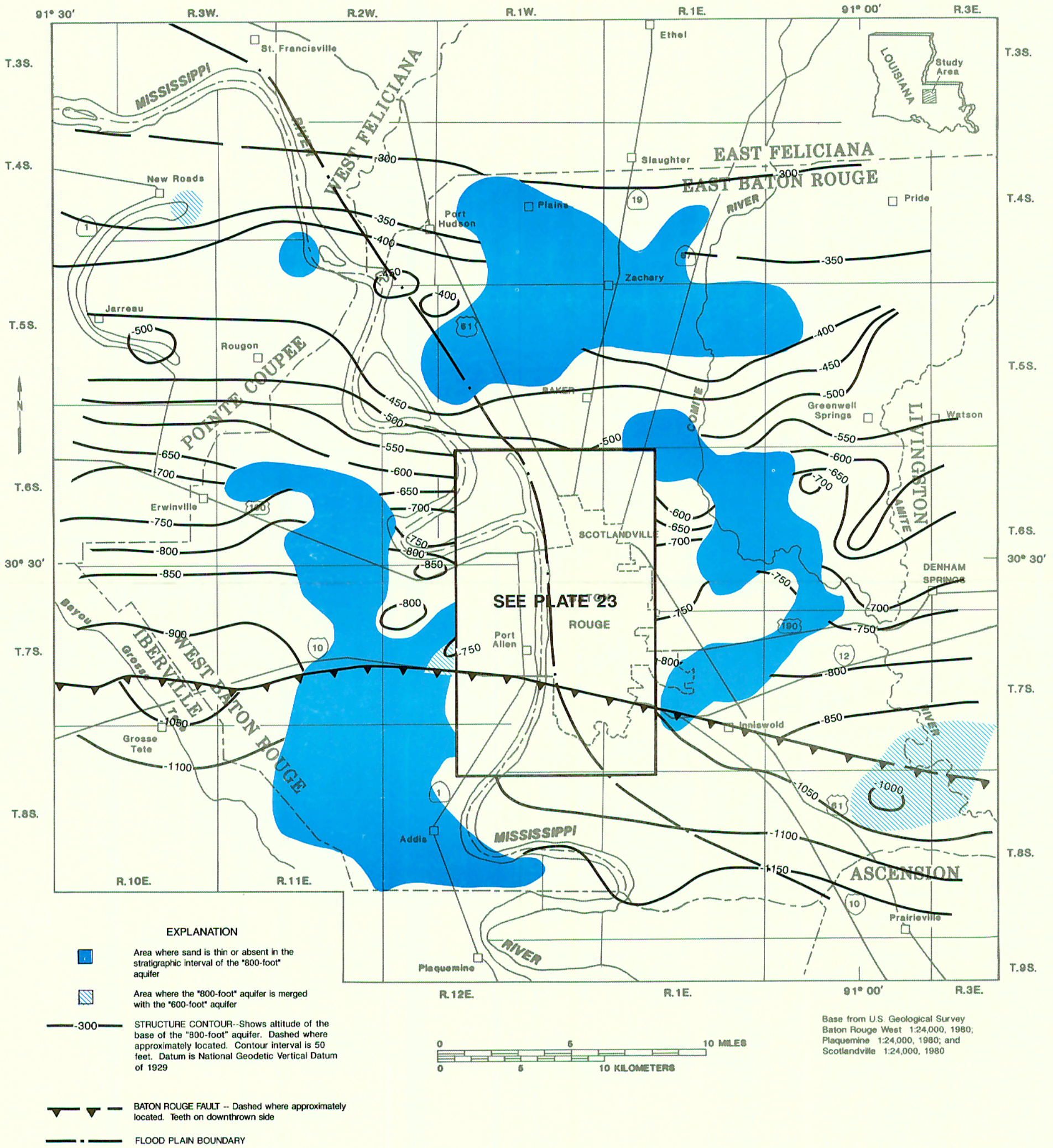
PLATE 24. ALTITUDE OF THE BASE OF THE "800-FOOT" AQUIFER IN EAST BATON ROUGE PARISH AND SURROUNDING PARISHES, LOUISIANA.
