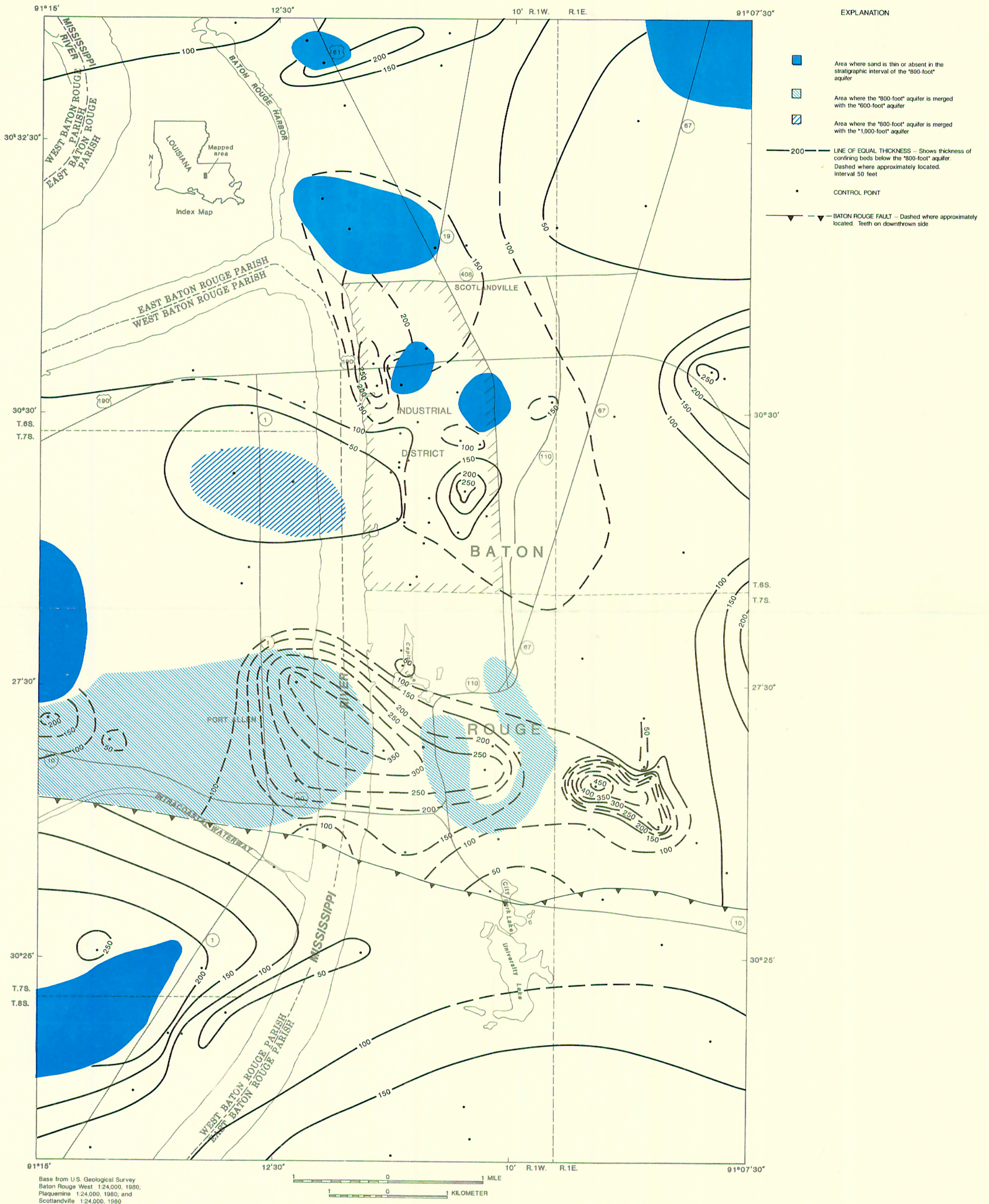
PLATE 27. CONFINING BED THICKNESS BELOW THE "800-FOOT" AQUIFER IN THE BATON ROUGE INDUSTRIAL DISTRICT AND THE SURROUNDING AREA, LOUISIANA.
