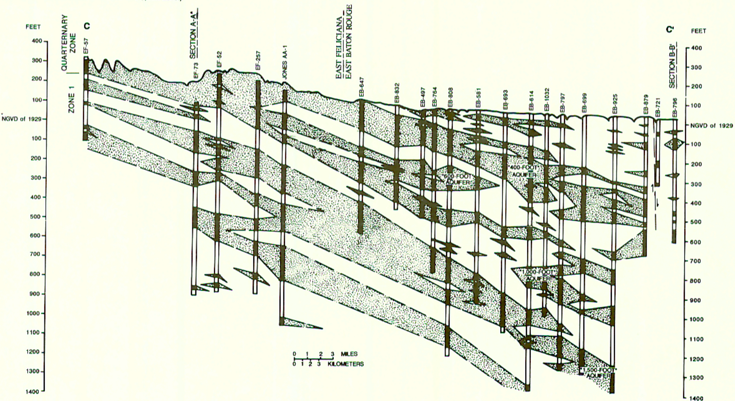
GEOHYDROLOGIC SECTIONS THROUGH EAST AND WEST BATON ROUGE, EAST AND WEST FELICIANA, POINTE COUPEE, AND ST. HELENA PARISHES, LOUISIANA.
