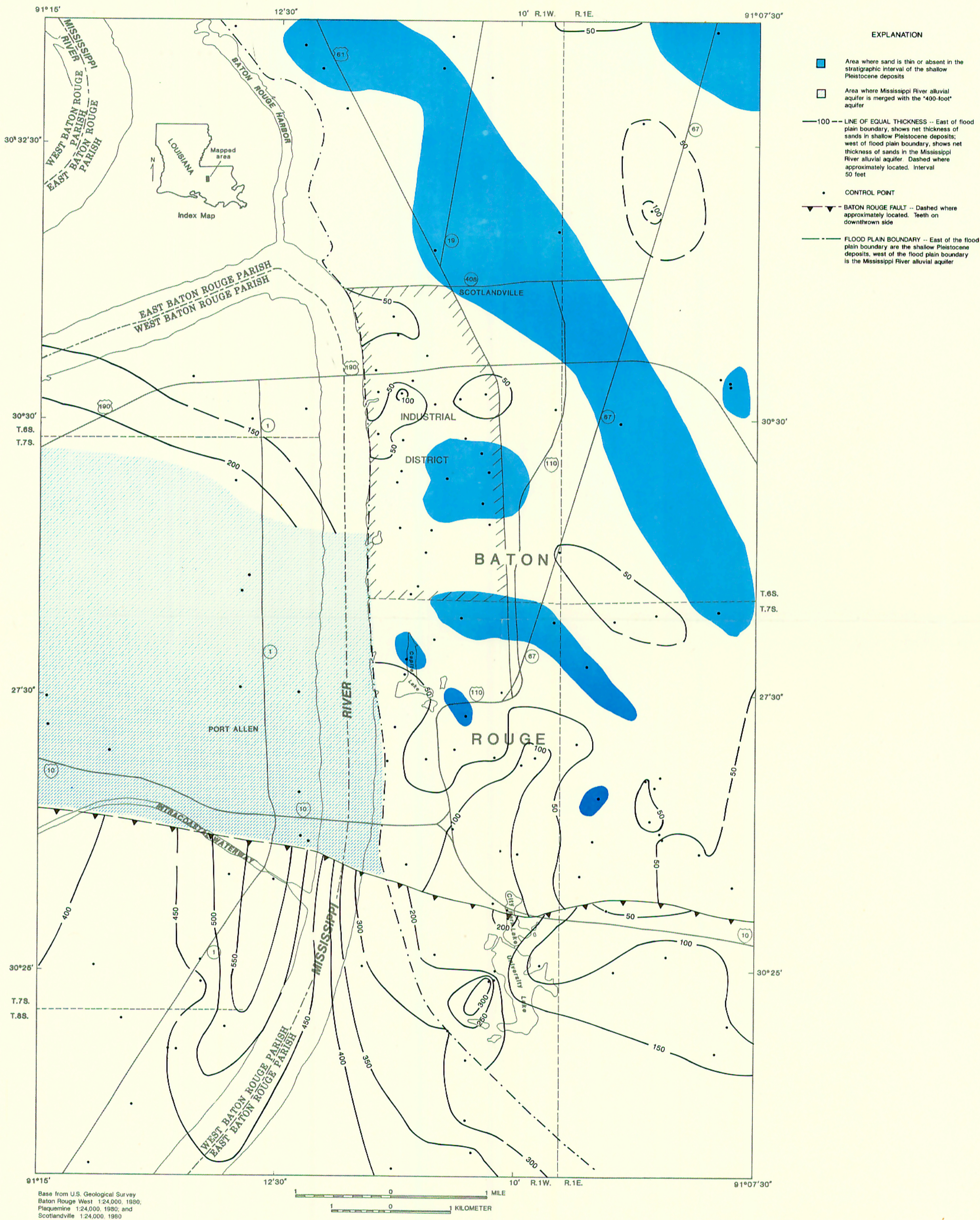
PLATE 7. NET SAND THICKNESS IN THE SHALLOW PLEISTOCENE DEPOSITS AND THE MISSISSIPPI RIVER ALLUVIAL AQUIFER IN THE BATON ROUGE INDUSTRIAL DISTRICT AND THE SURROUNDING AREA, LOUISIANA.
