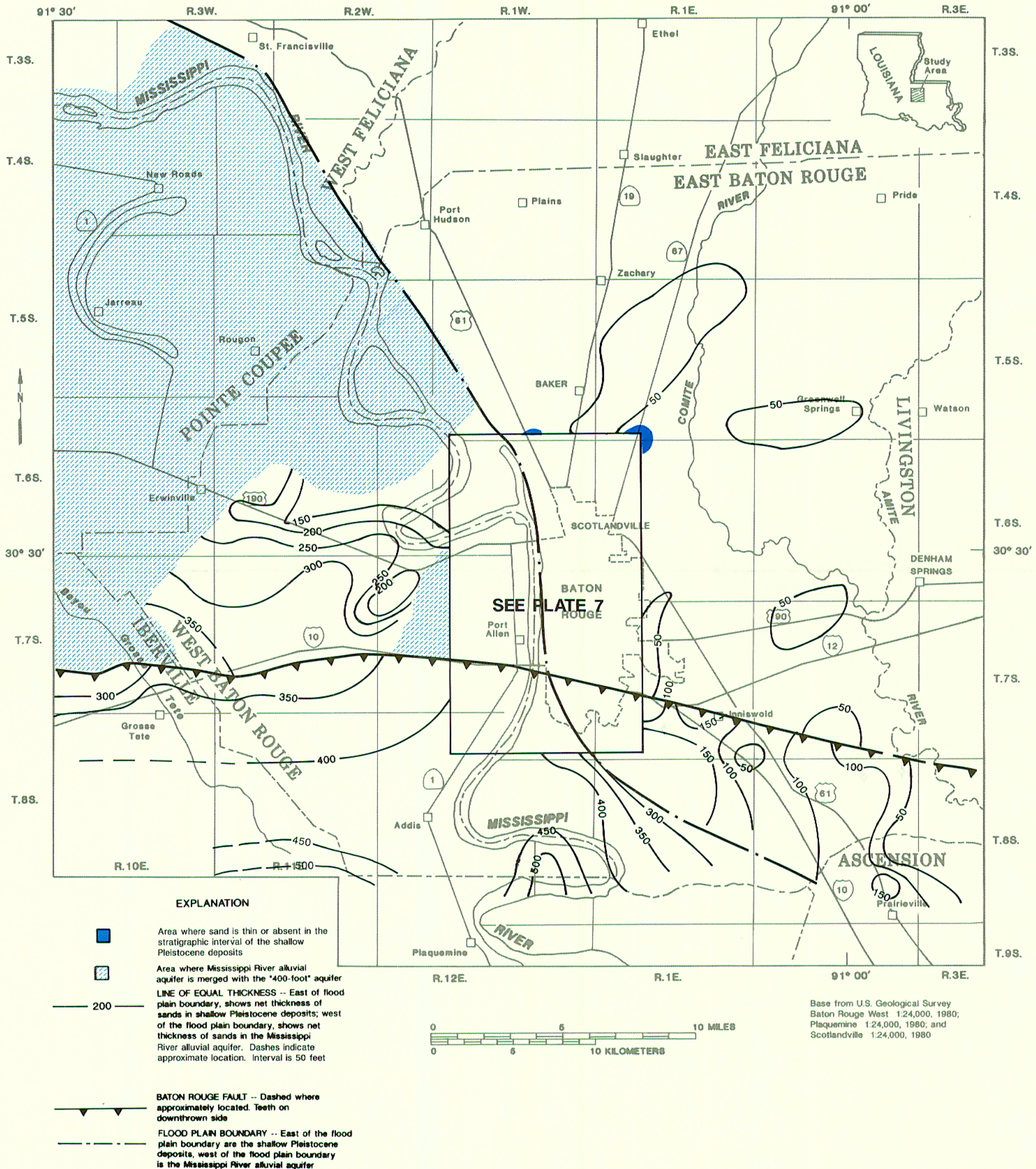
PLATE 8. NET SAND THICKNESS IN SHALLOW PLEISTOCENE DEPOSITS AND THE MISSISSIPPI RIVER ALLUVIAL AQUIFER IN EAST BATON ROUGE PARISH AND THE SURROUNDING PARISHES, LOUISIANA.
