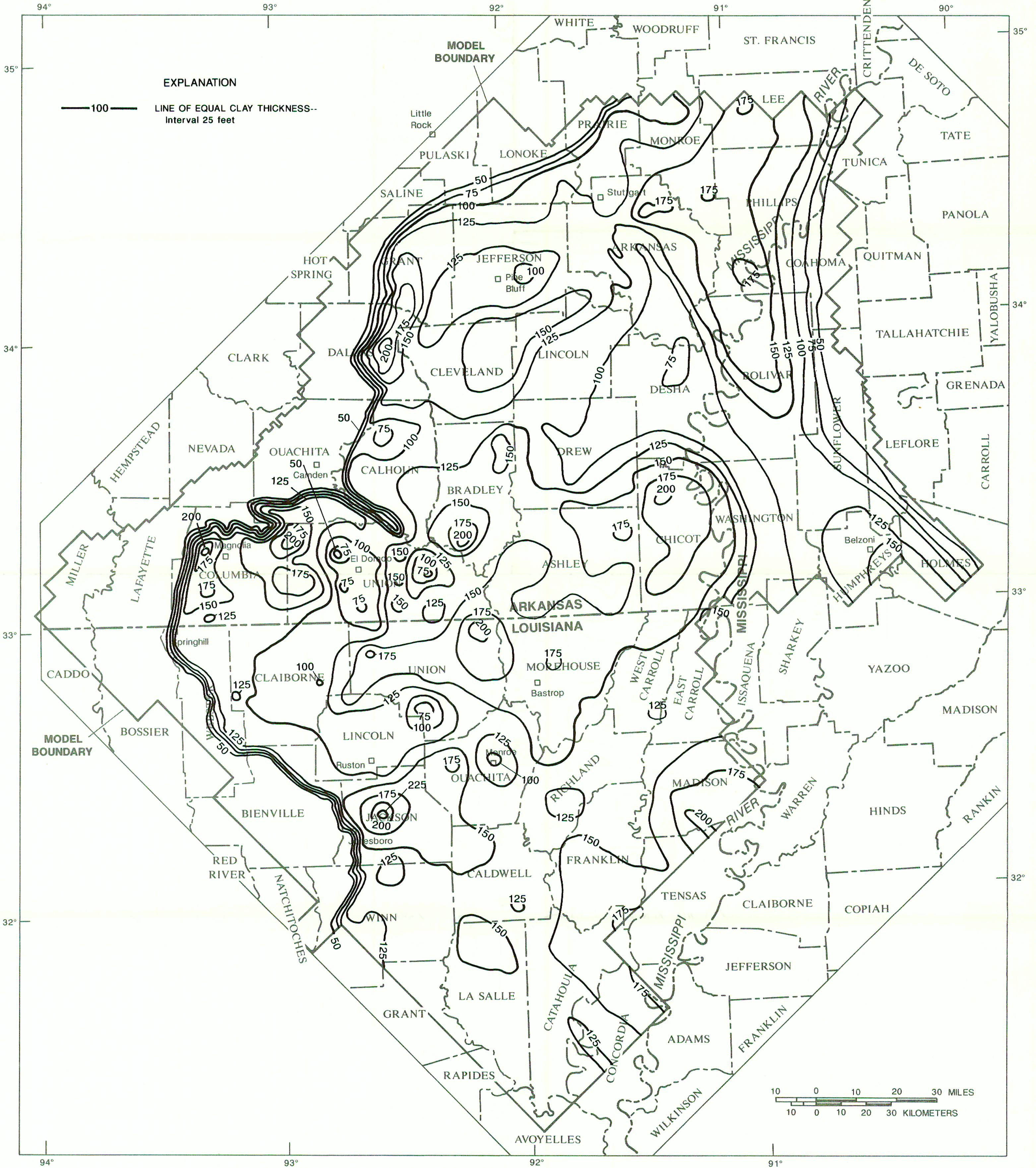
CLAY THICKNESS WITHIN THE COOK MOUNTAIN CONFINING UNIT, NORTHERN LOUISIANA, SOUTHERN ARKANSAS, AND NORTHWESTERN MISSISSIPPI.
