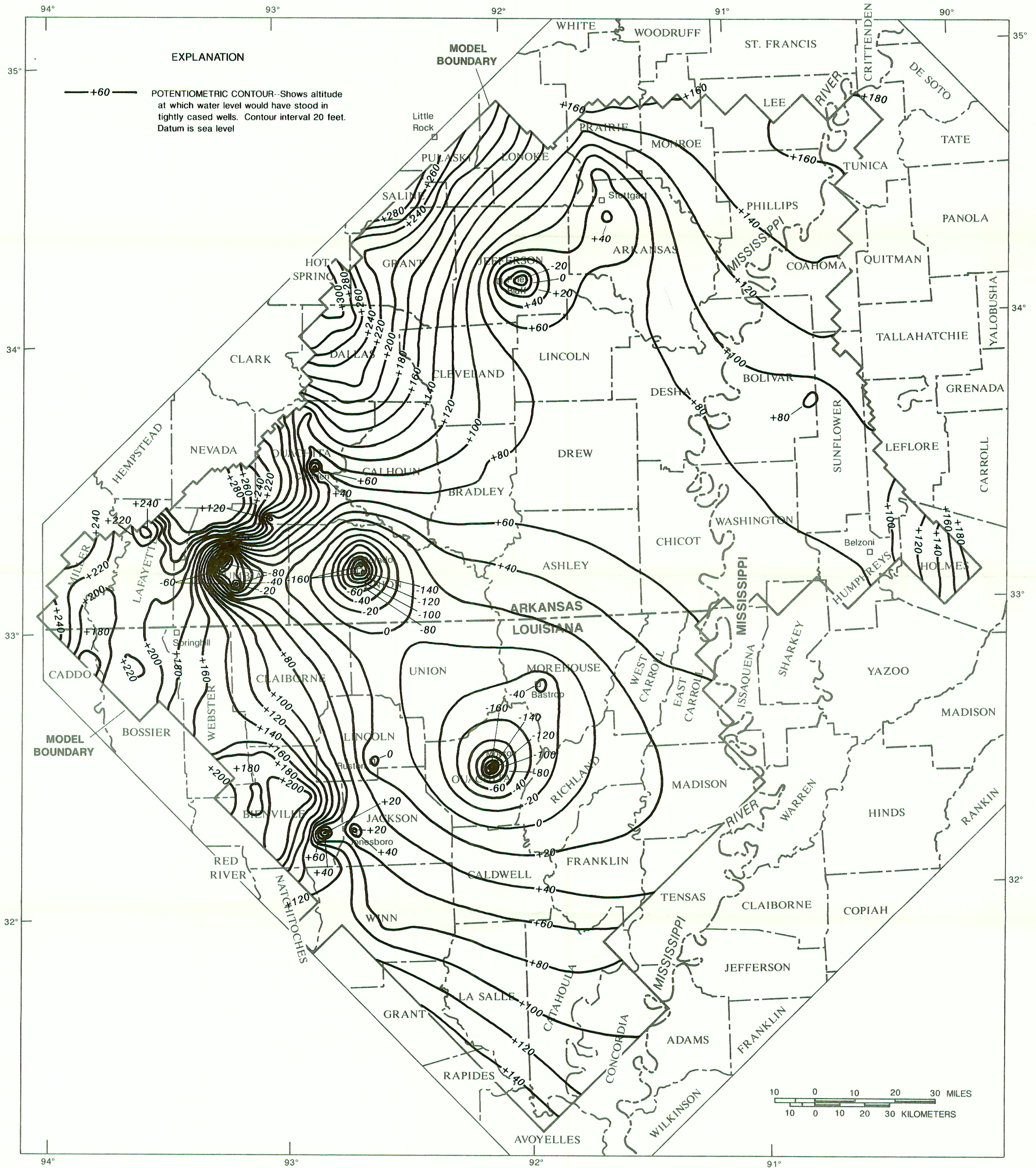
SIMULATED POTENTIOMETRIC SURFACE OF THE SPARTA AQUIFER, 1985, NORTHERN LOUISIANA, SOUTHERN ARKANSAS, AND NORTHWESTERN MISSISSIPPI.
