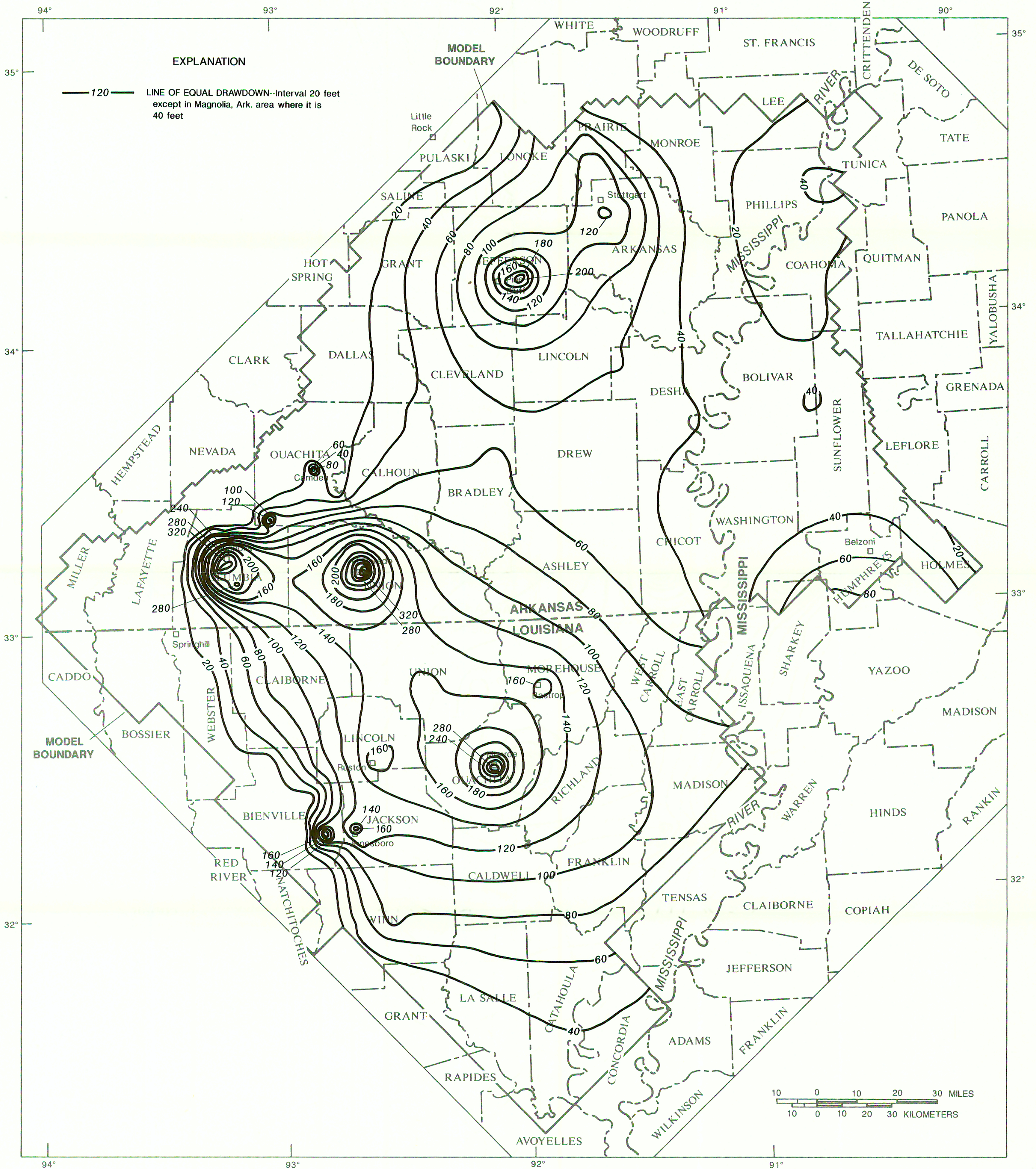
SIMULATED DRAWDOWN, PREDEVELOPMENT TO 1985, NORTHERN LOUISIANA, SOUTHERN ARKANSAS, AND NORTHWESTERN MISSISSIPPI.
