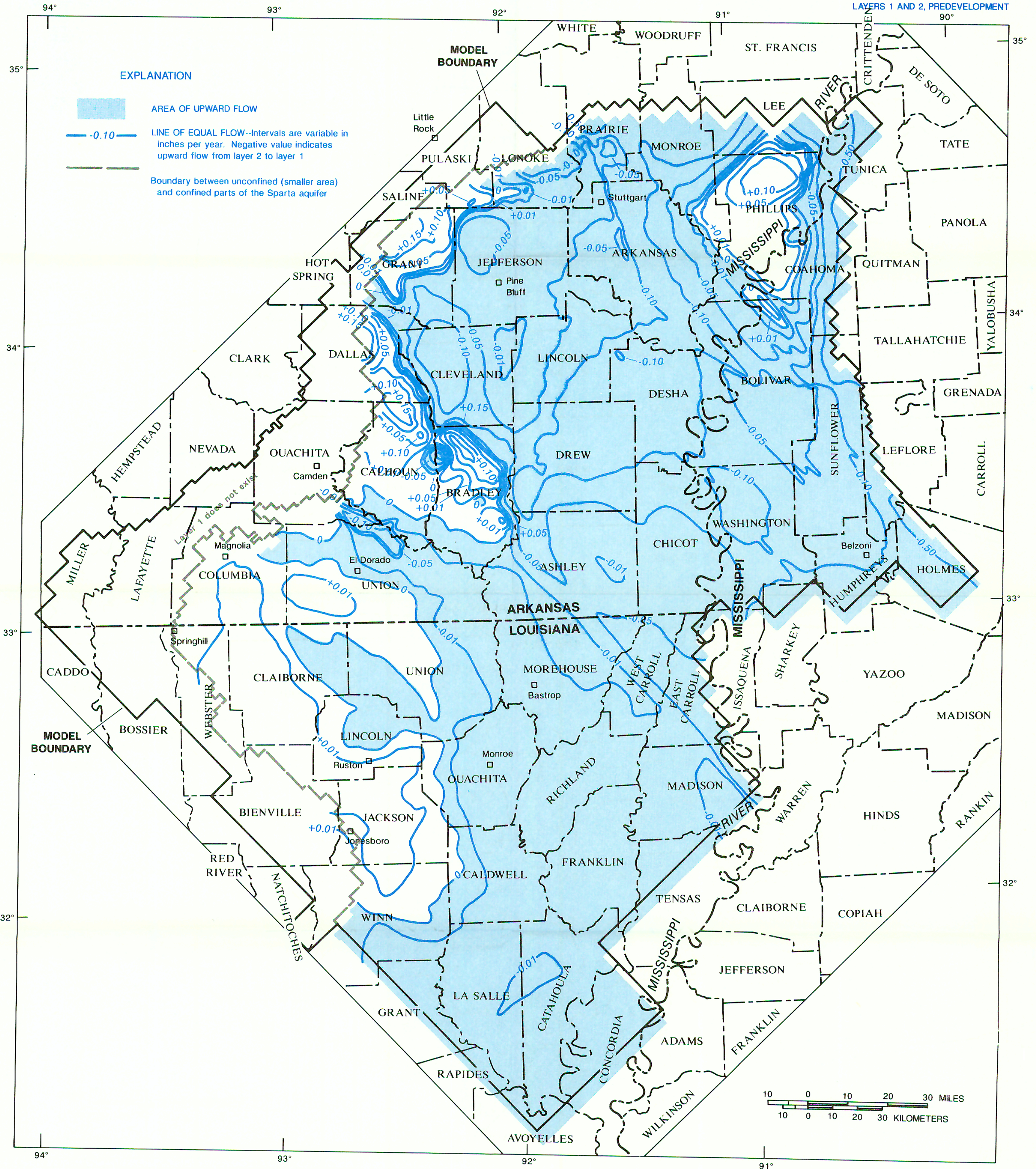
SIMULATED FLOW BETWEEN LAYER 1 AND LAYER 2, PREDEVELOPMENT, NORTHERN LOUISIANA, SOUTHERN ARKANSAS, AND NORTHWESTERN MISSISSIPPI.
