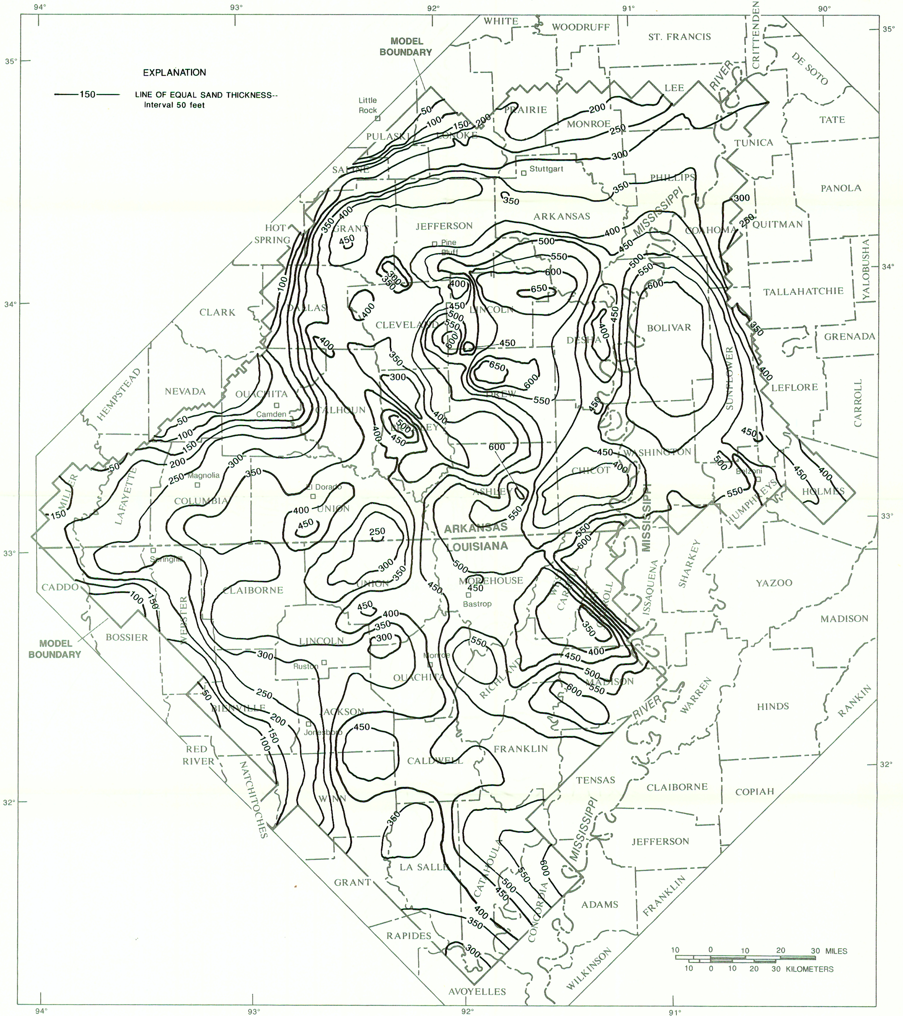
SAND THICKNESS WITHIN THE SPARTA AQUIFER, NORTHERN LOUISIANA, SOUTHERN ARKANSAS, AND NORTHWESTERN MISSISSIPPI.
