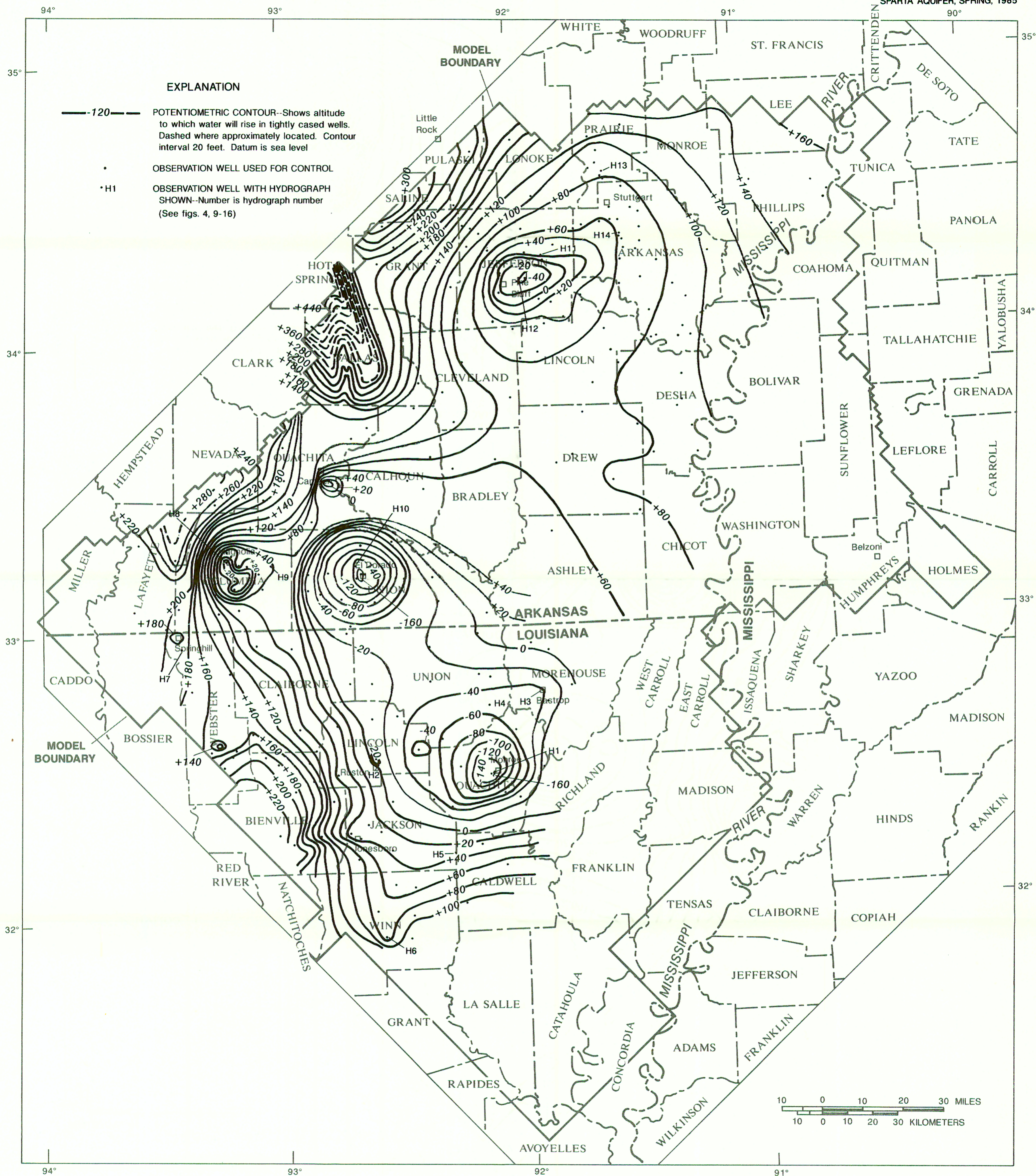
POTENTIOMETRIC SURFACE OF THE SPARTA AQUIFER, SPRING, 1985, NORTHERN LOUISIANA, SOUTHERN ARKANSAS, AND NORTHWESTERN MISSISSIPPI.
