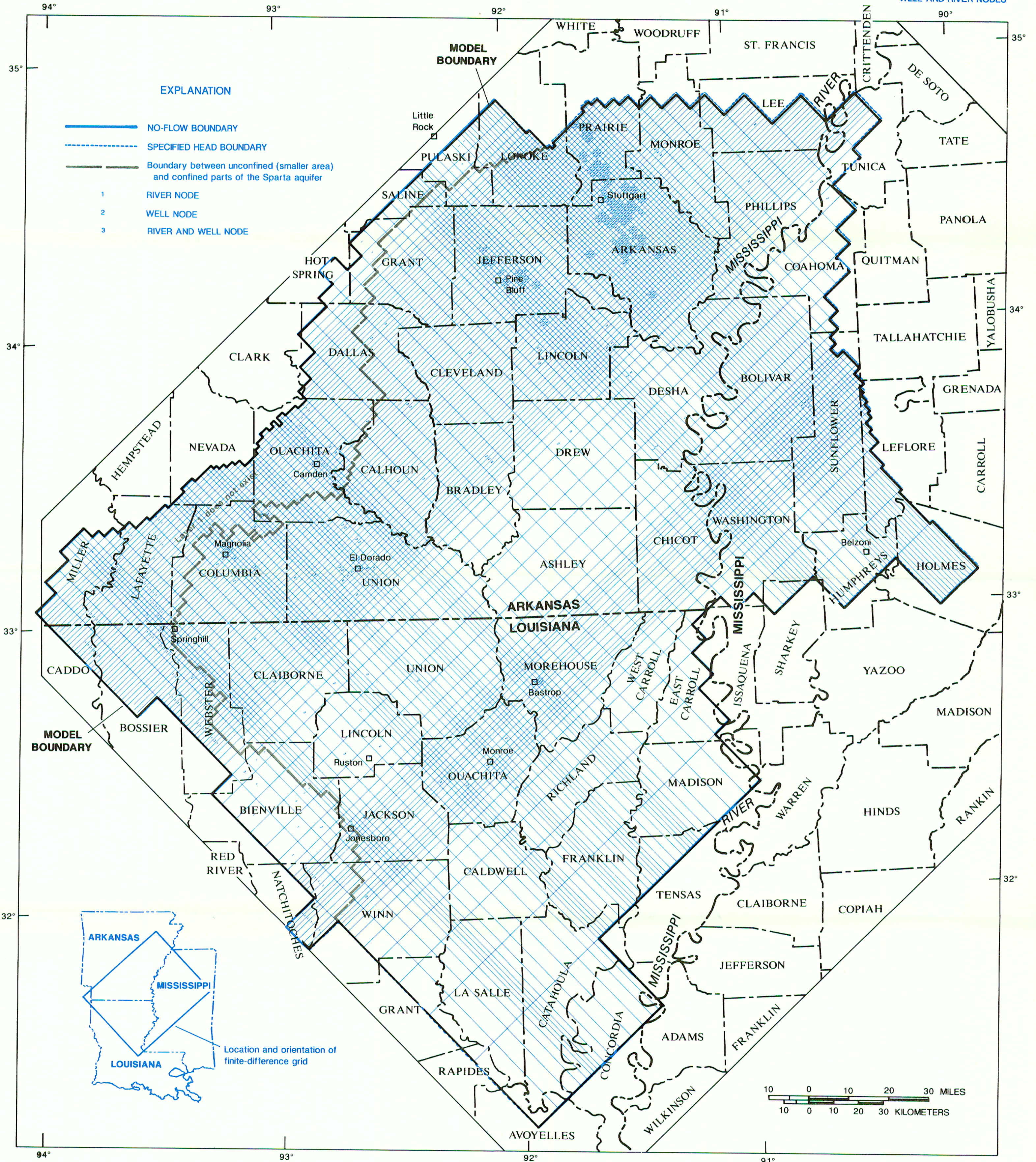
BOUNDARIES, AND WELL AND RIVER NODES FOR LAST STRESS PERIOD (1983-85) OF THE MODEL, NORTHERN LOUISIANA, SOUTHERN ARKANSAS, AND NORTHWESTERN MISSISSIPPI.
