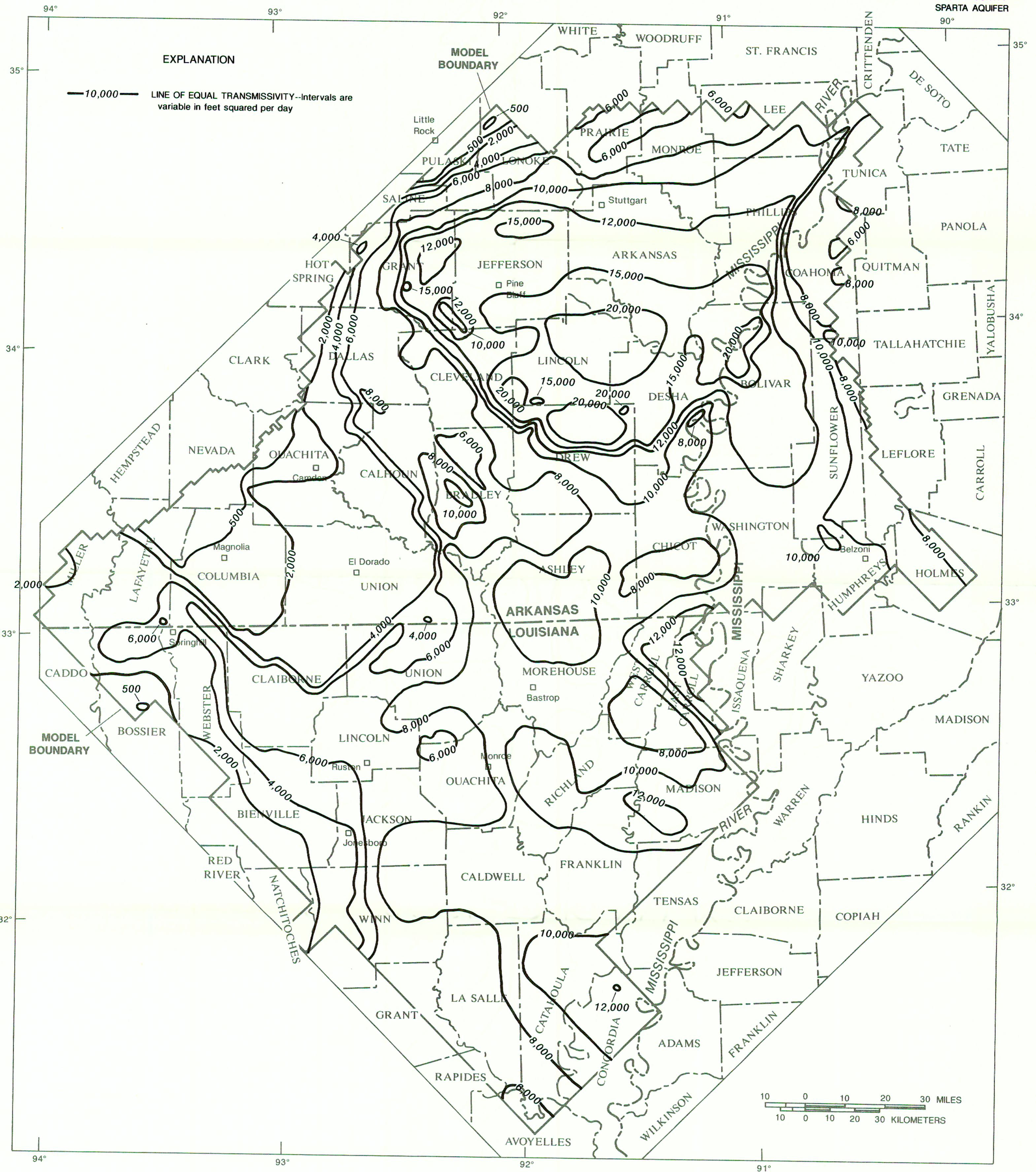
MODEL-DERIVED TRANSMISSIVITY OF THE SPARTA AQUIFER, NORTHERN LOUISIANA, SOUTHERN ARKANSAS, AND NORTHWESTERN MISSISSIPPI.
