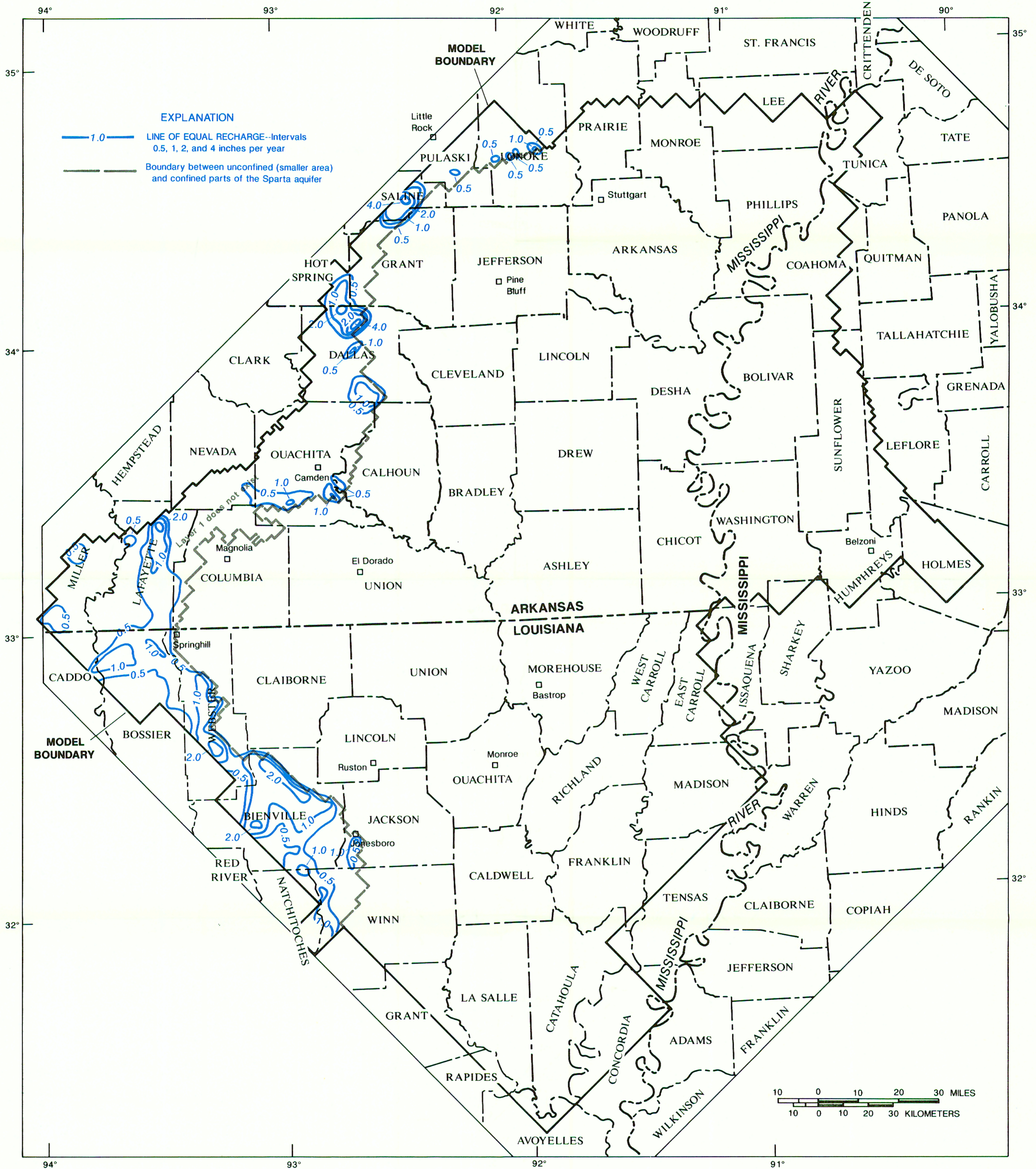
MODEL-DERIVED RECHARGE TO THE SPARTA AQUIFER, NORTHERN LOUISIANA, SOUTHERN ARKANSAS, AND NORTHWESTERN MISSISSIPPI.
