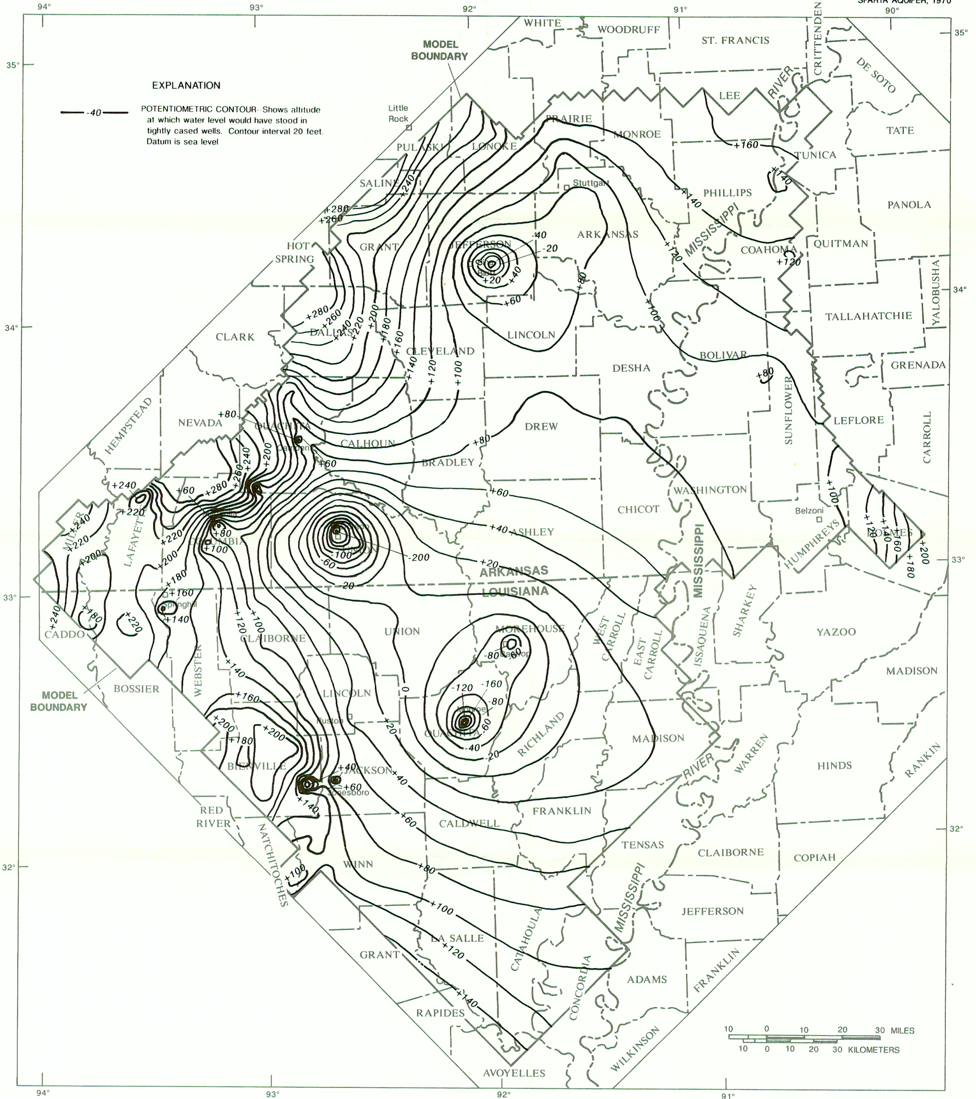
SIMULATED POTENTIOMETRIC SURFACE OF THE SPARTA AQUIFER, 1970, NORTHERN LOUISIANA, SOUTHERN ARKANSAS, AND NORTHWESTERN MISSISSIPPI.
