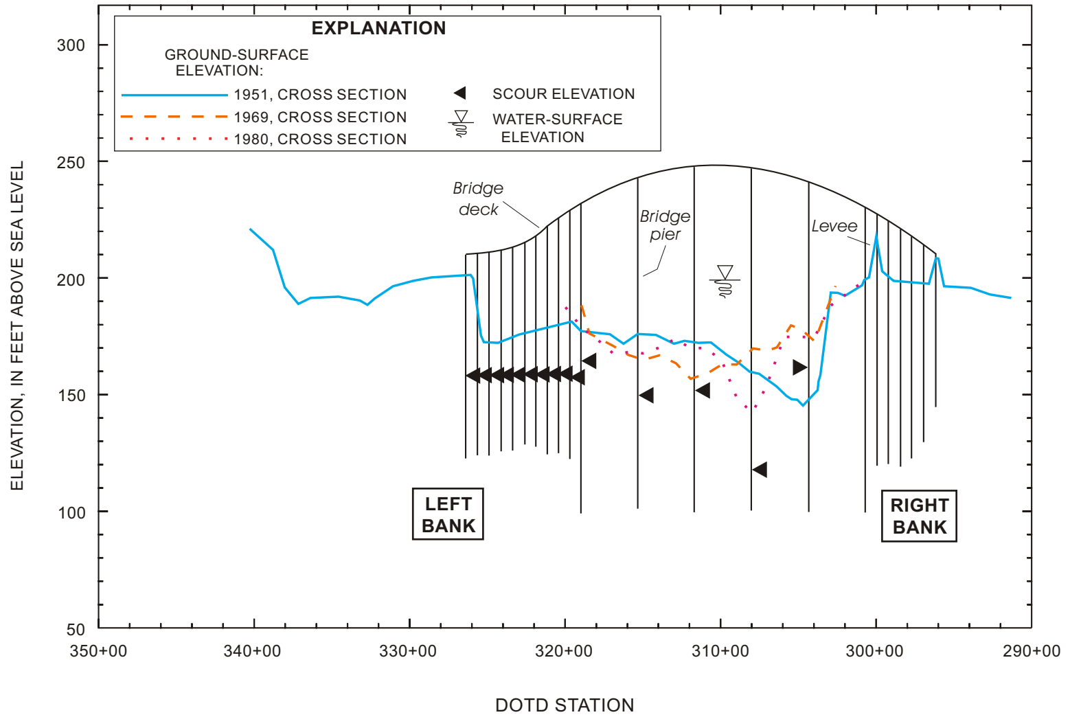
Figure 39. Comparative cross sections and pier-scour estimates at Louisiana Highway 2 crossing near Hosston, Louisiana (revised 1999).
