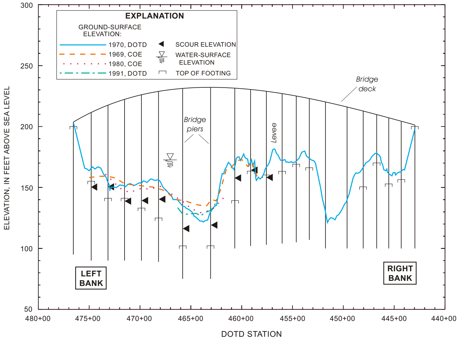
Figure 36. Comparative cross sections and pier-scour estimates at Interstate Highway 220 crossing at Shreveport, Louisiana (revised 1999).
