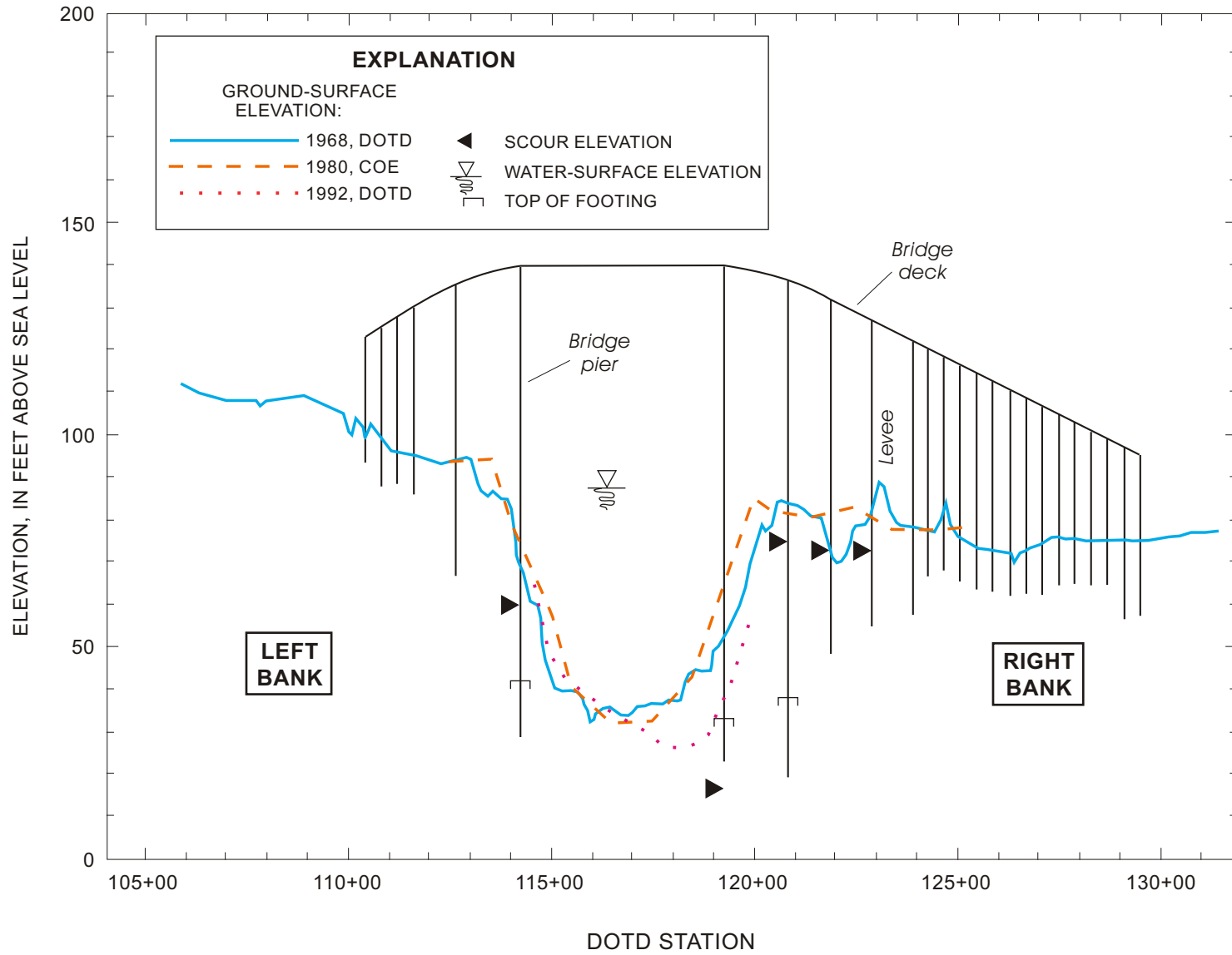
Figure 12. Comparative cross sections and pier-scour estimates at U.S. Highway 71 crossing at Alexandria, Louisiana.
