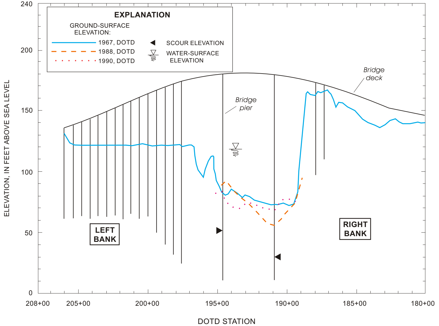
Figure 18. Comparative cross sections and pier-scour estimates at Louisiana Highway 6 crossing at Grand Ecore, Louisiana (revised 1999).
