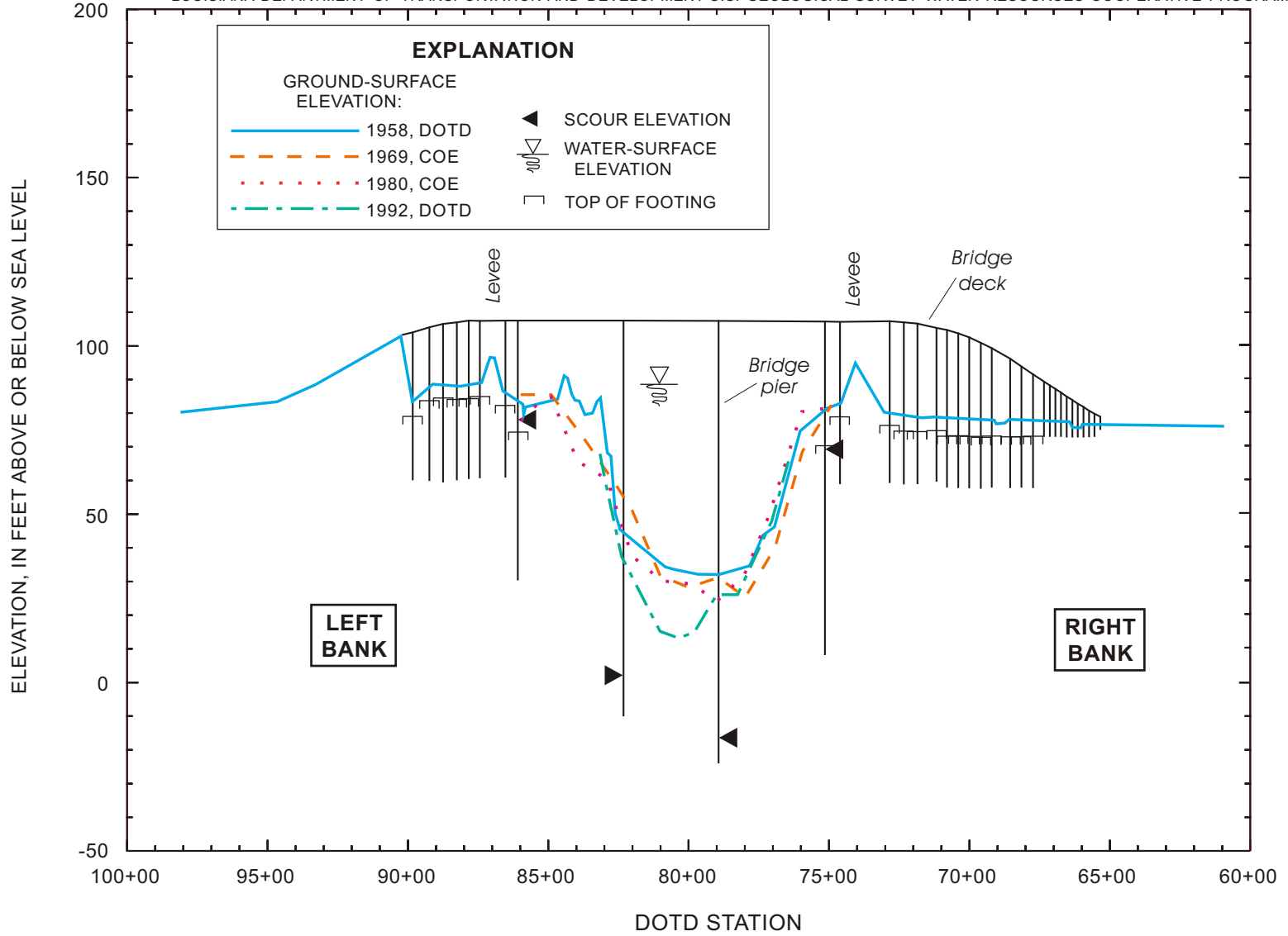
Figure 7. Comparative cross sections and pier-scour estimates at U.S. Highway 167 crossing at Alexandria, Louisiana (revised 1999).
