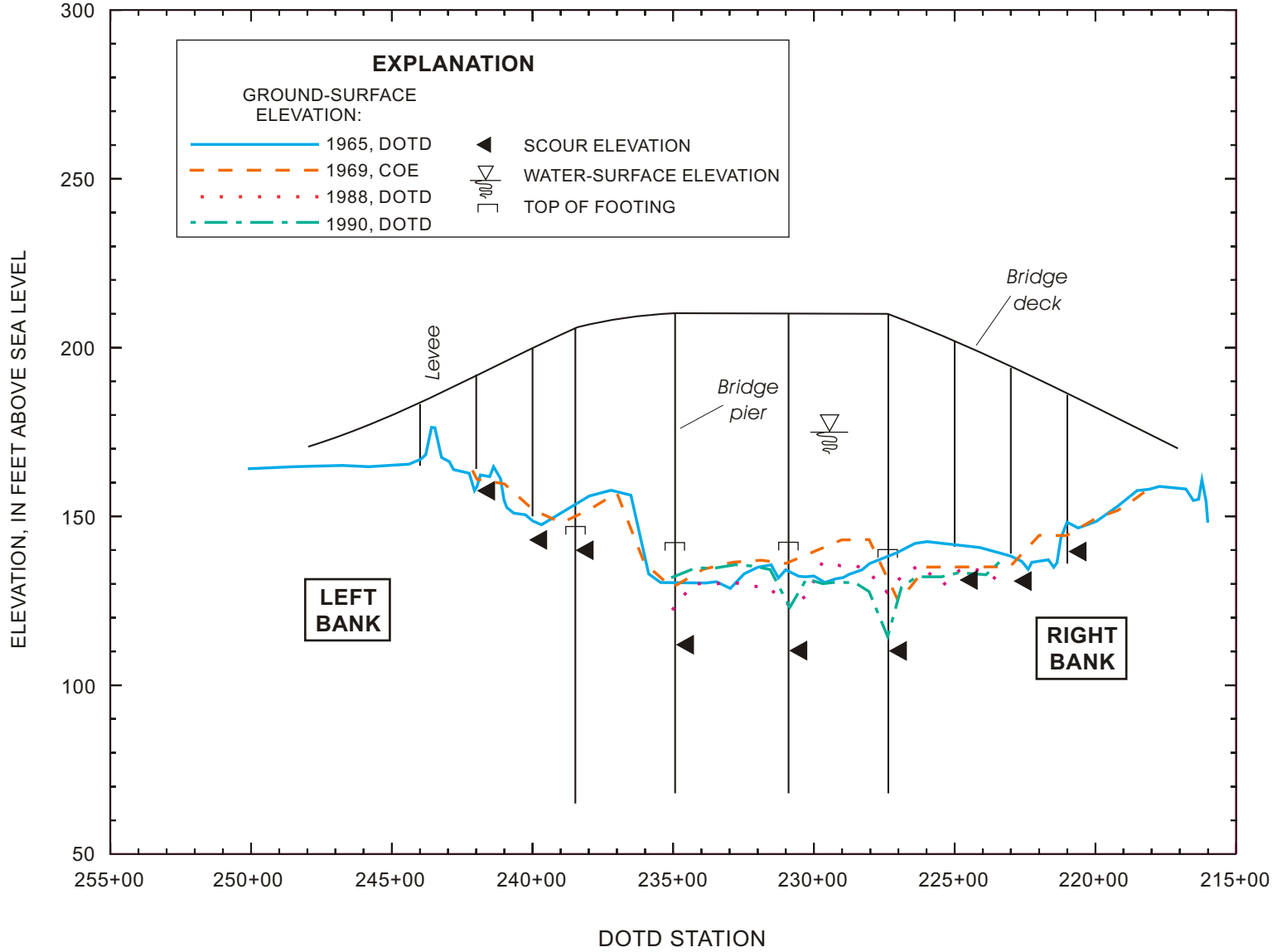
Figure 24. Comparative cross sections and pier-scour estimates at Louisiana Highway 511 crossing at Shreveport, Louisiana.
