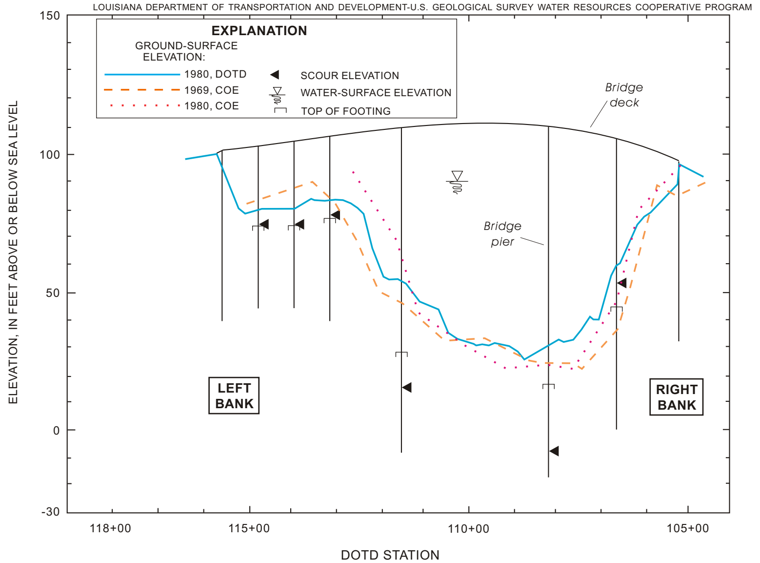
Figure 9. Comparative cross sections and pier-scour estimates at U.S. Highway 165 crossing at Alexandria, Louisiana (revised 1999).
