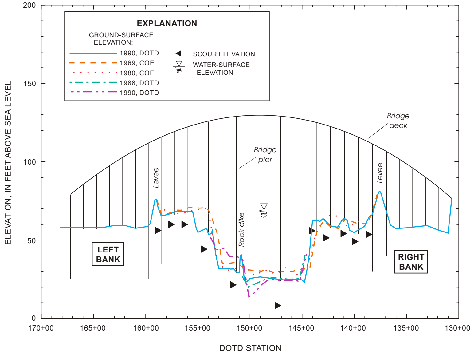
Figure 4. Comparative cross sections and pier-scour estimates at Louisiana Highway 107 crossing near Moncla, Louisiana.
