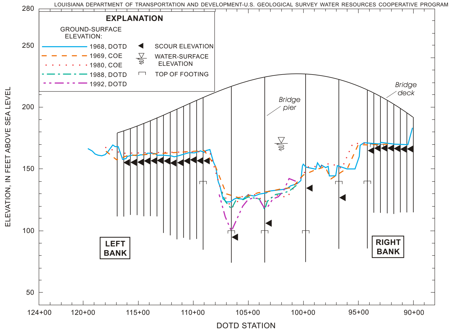
Figure 27. Comparative cross sections and pier-scour estimates at Louisiana Highway 3032 crossing at Shreveport, Louisiana.
