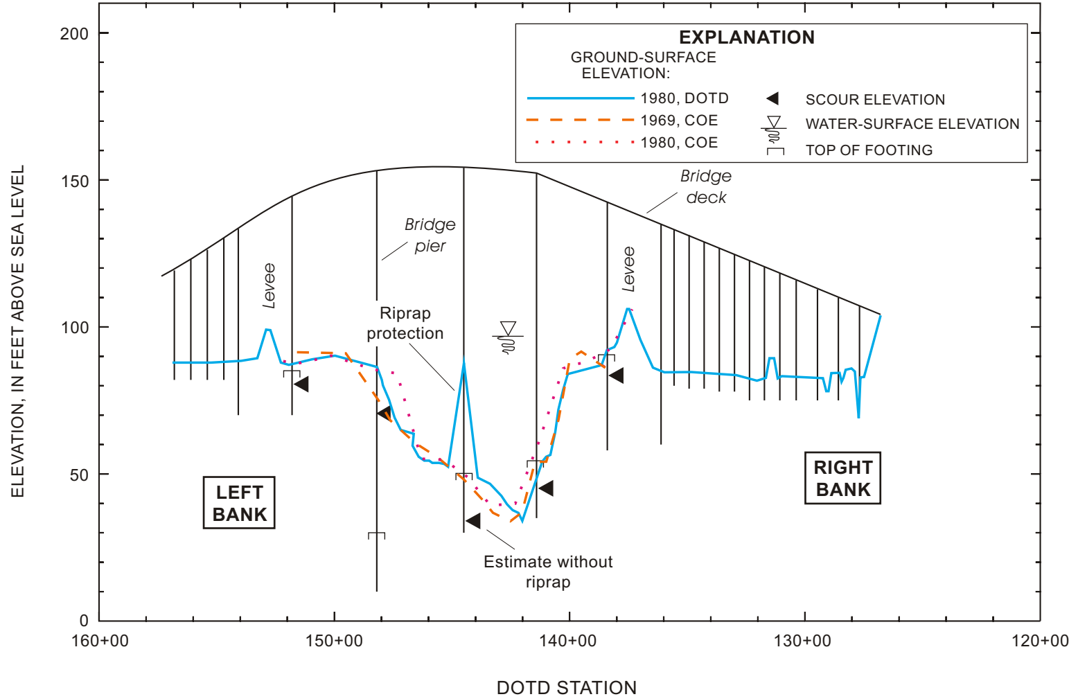
Figure 15. Comparative cross sections and pier-scour estimates at Louisiana Highway 8 crossing at Boyce, Louisiana (revised 1999).
