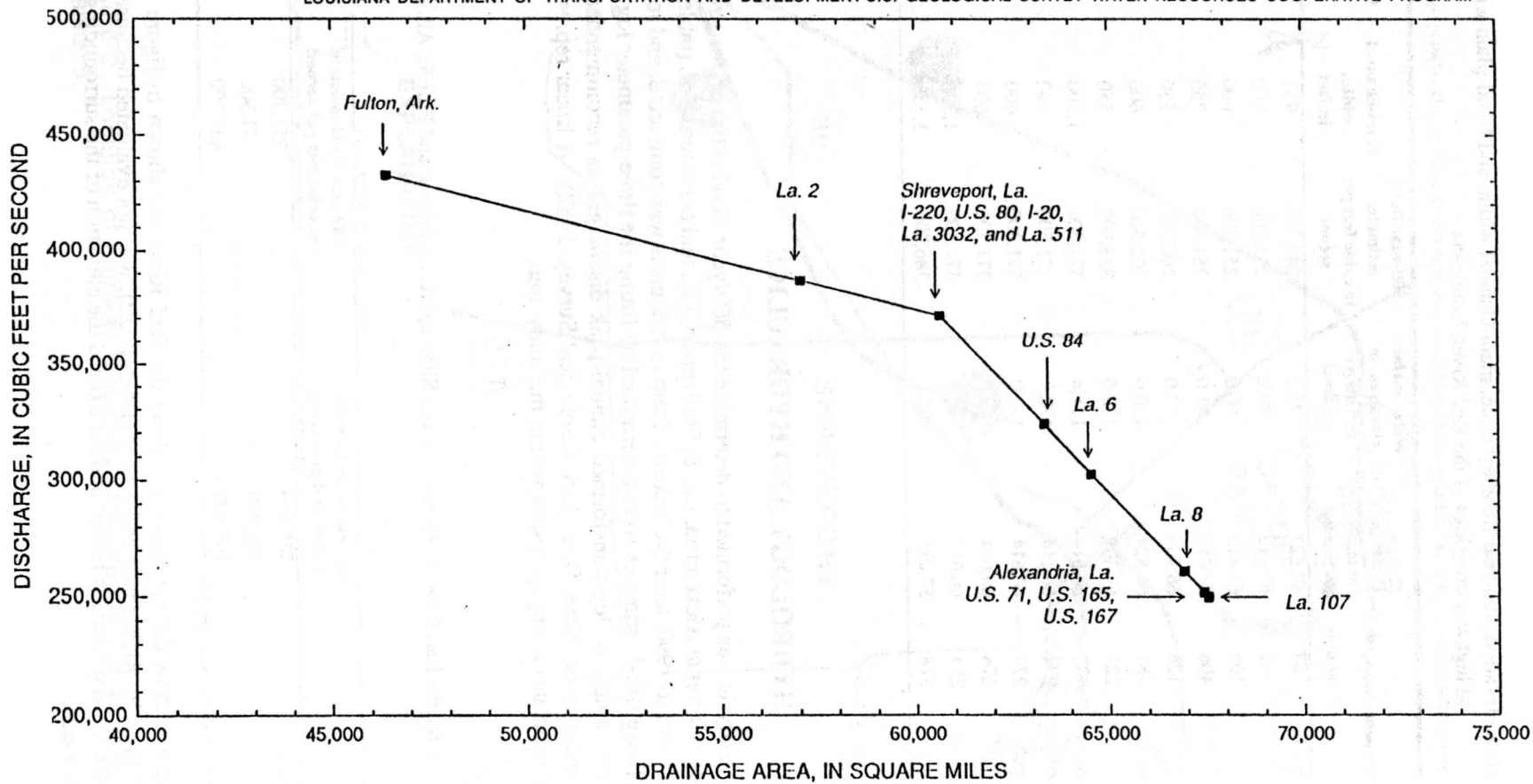
Figure 3. The 500-year flood estimates on the Red River from Fulton, Arkansas, to Alexandria, Louisiana.
