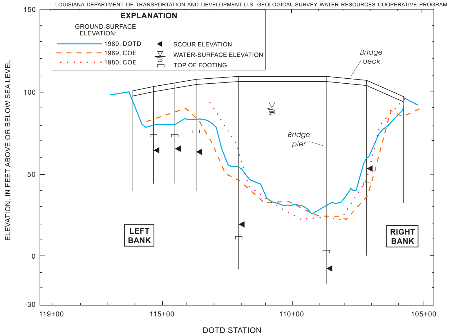
Figure 8. Comparative cross sections and pier-scour estimates at U.S. Highway 167 bridge at Alexandria, Louisiana.
