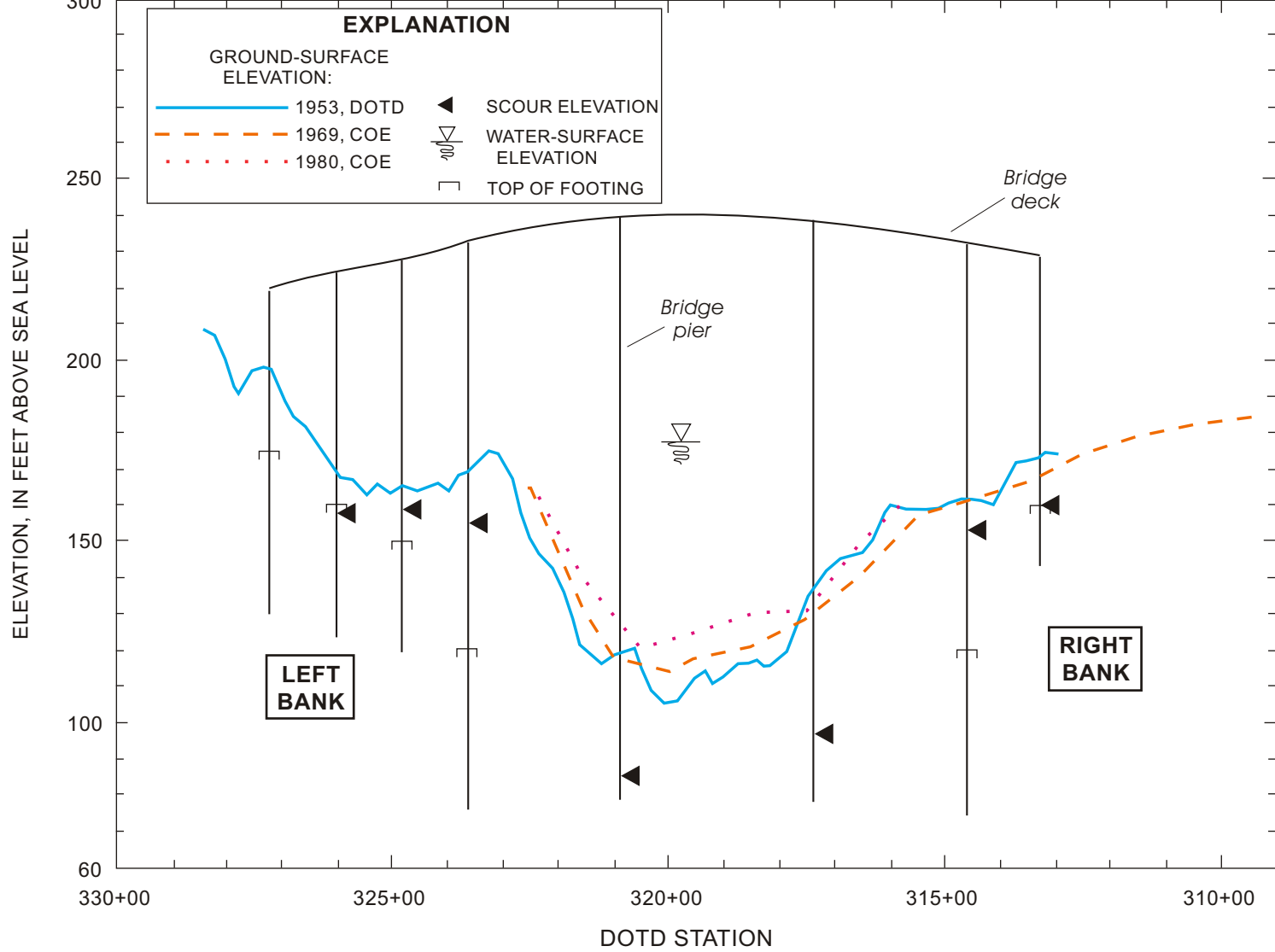
Figure 30. Comparative cross sections and pier-scour estimates at Interstate Highway 20 crossing at Shreveport, Louisiana.
