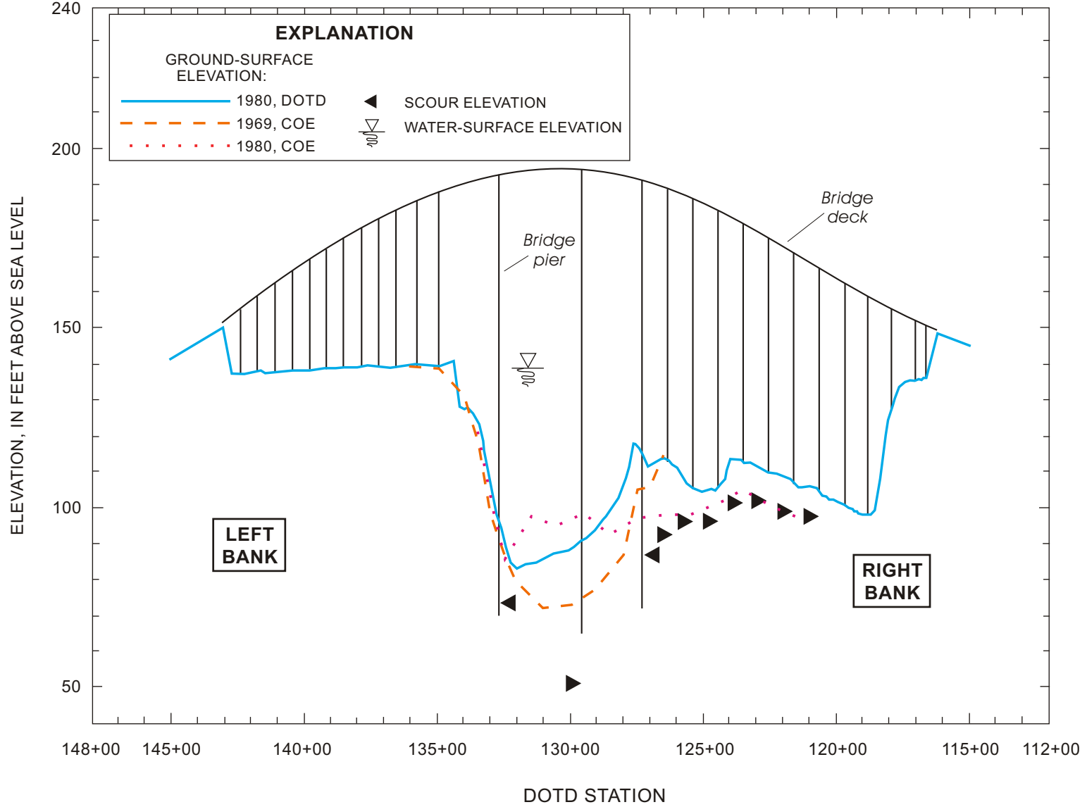
Figure 21. Comparative cross sections and pier-scour estimates at U.S. Highway 84 crossing at Coushatta, Louisiana.
