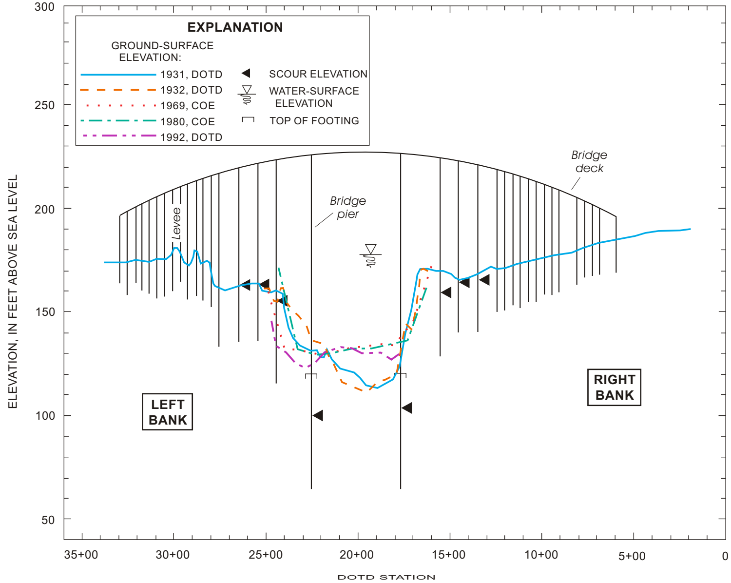
Figure 33. Comparative cross sections and pier-scour estimates at U.S. Highway 80 crossing at Shreveport, Louisiana (revised 1999).
