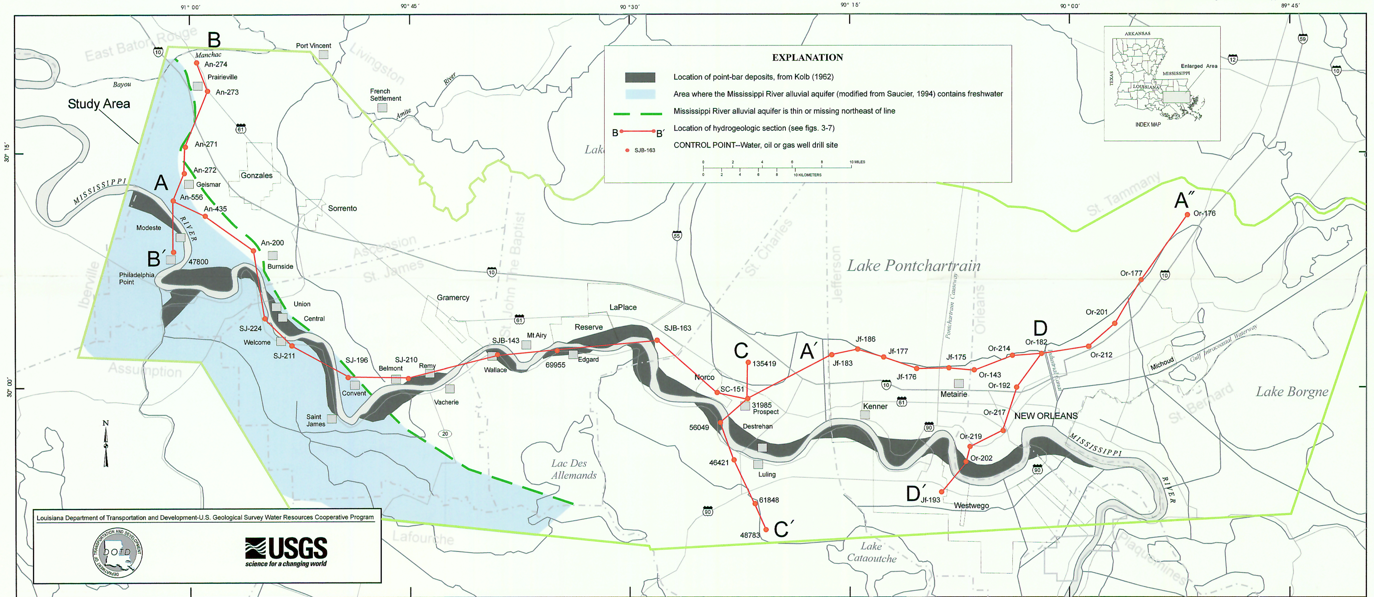
Plate 1. Location of point-bar deposits and distribution of freshwater in the Mississippi River alluvial aquifer, lower Mississippi River area in southeastern Louisiana.
