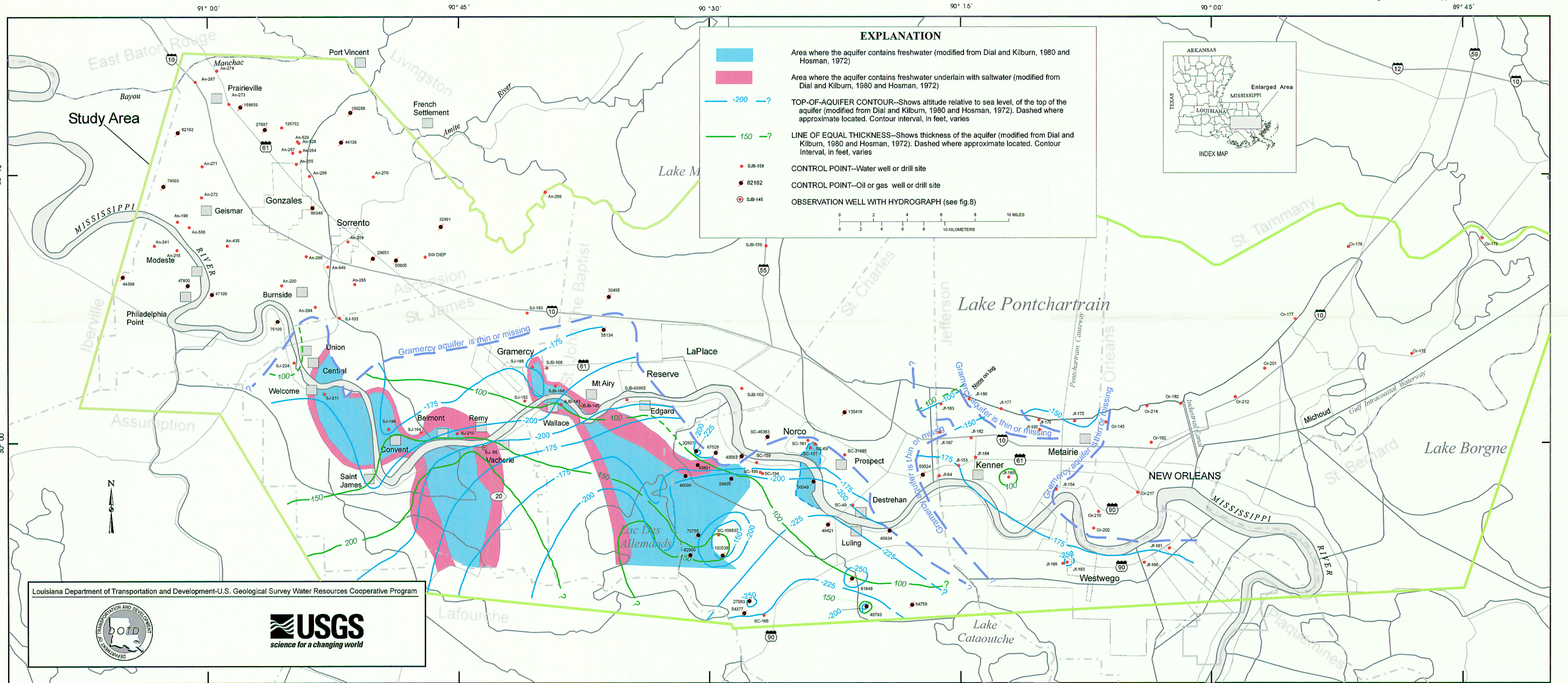
Plate 2. Altitude of top, extent and thickness, and distribution of freshwater in the Gramercy aquifer, lower Mississippi River area in southeastern Louisiana.
