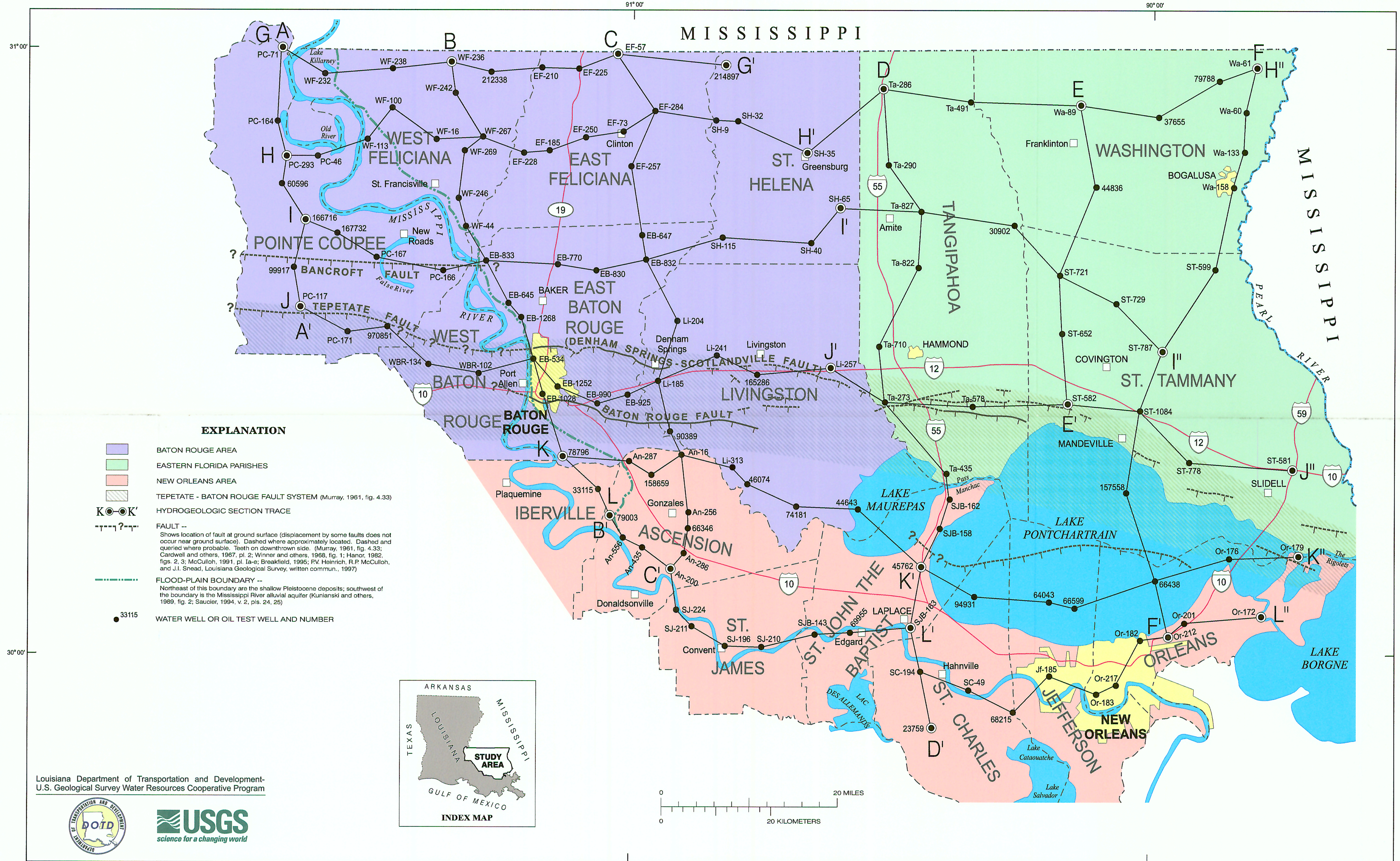
Plate 1. Location of study area and trace of hydrogeologic sections, southeastern Louisiana.
