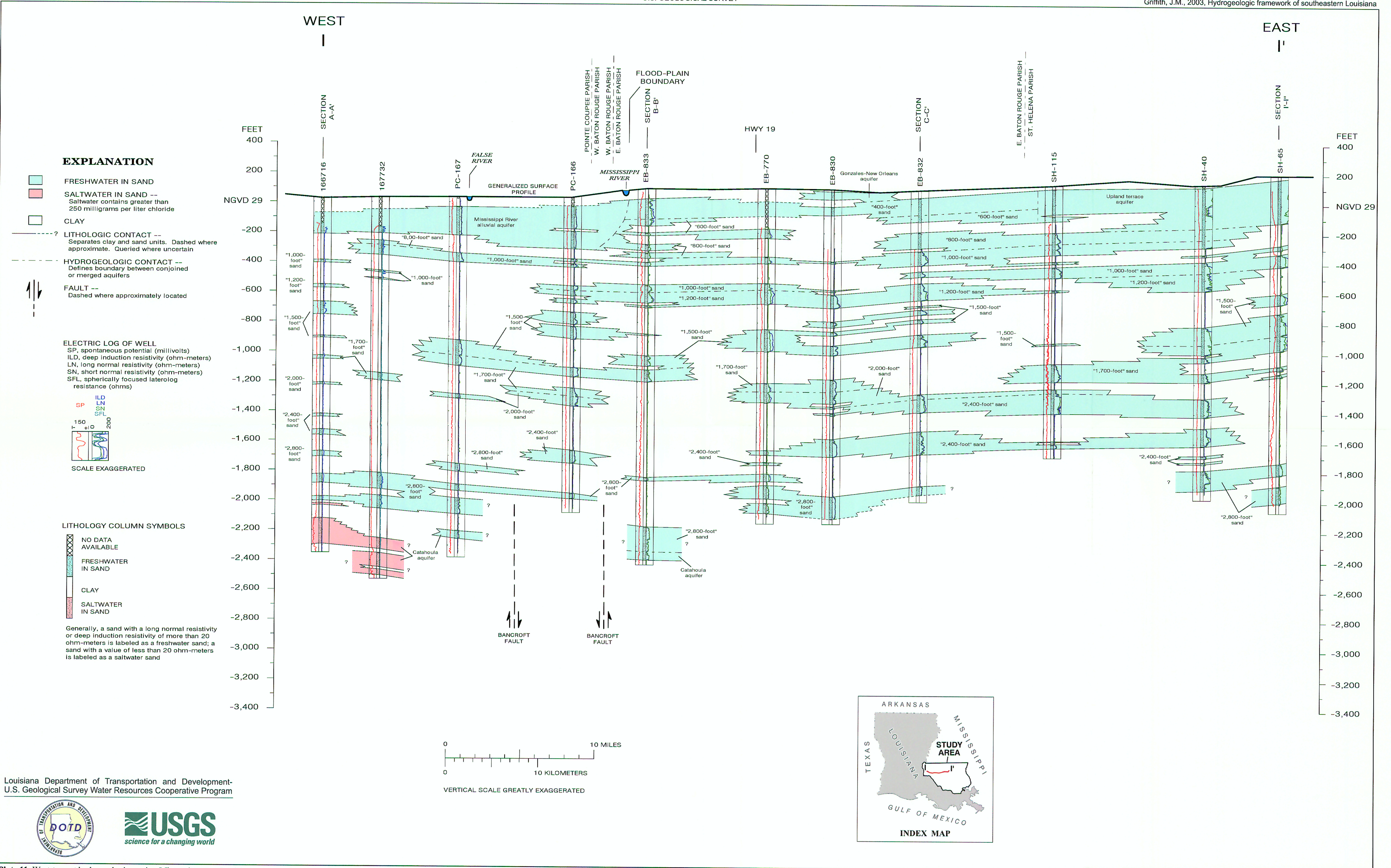
Plate 11. West-to-east hydrogeologic section I-I', southeastern Louisiana.
