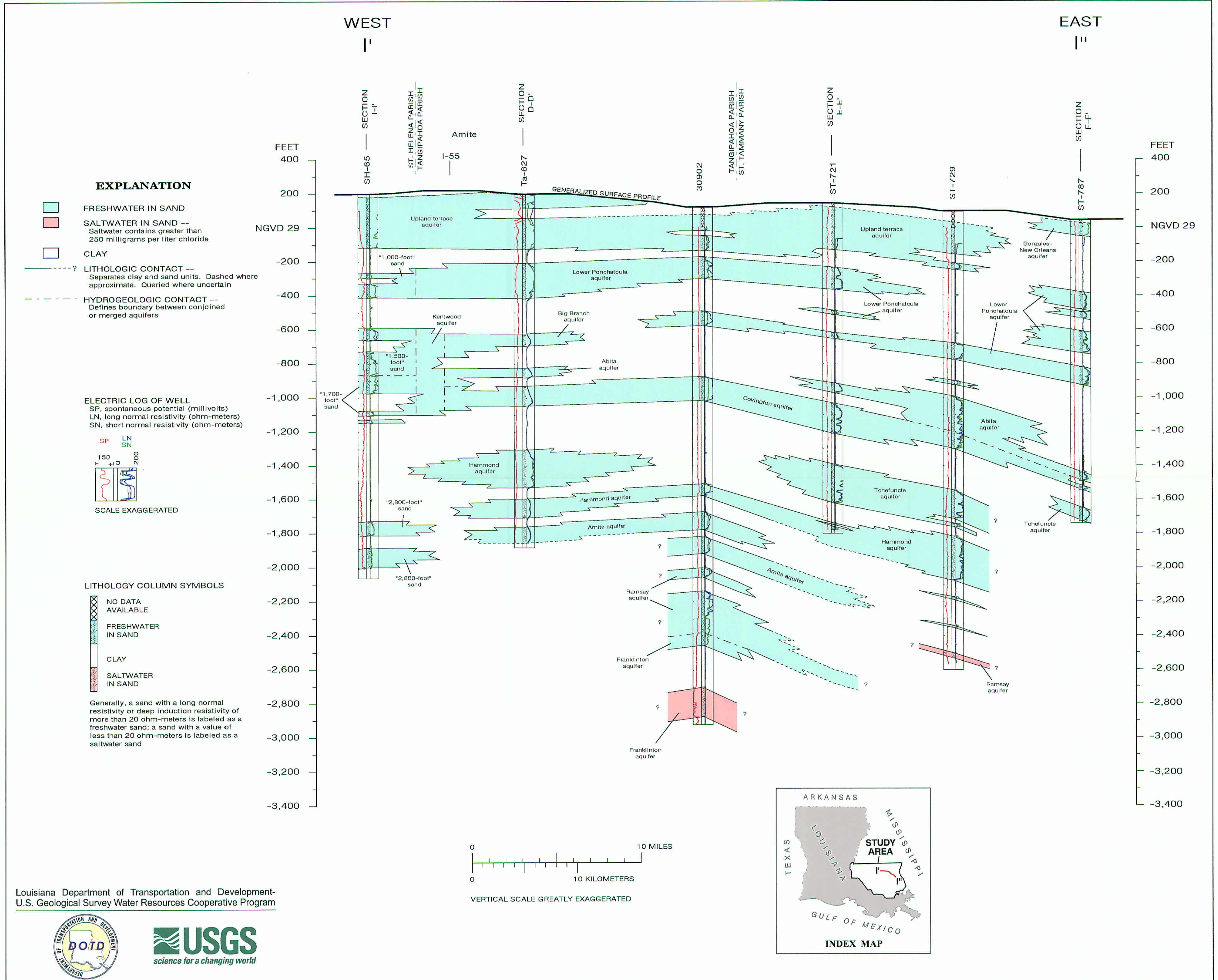
Plate 12. West-to-east hydrogeologic section I'-I'', southeastern Louisiana.
